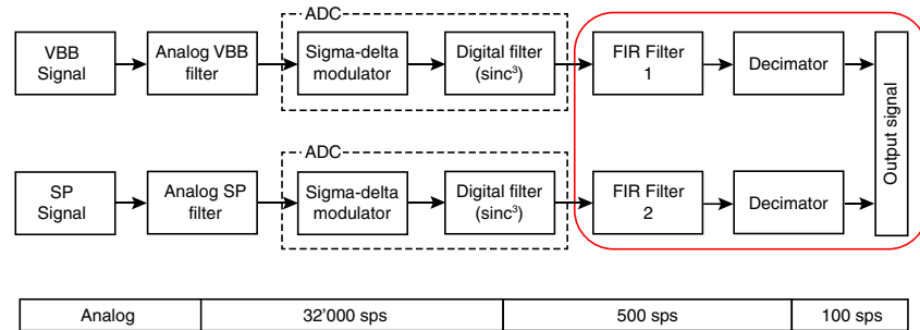
Figure 3. Acquisition and digitization of seismic signals recorded by the two SEIS seismometers. The filtering step in the red box can be changed from Earth by uploading different filter coefficients to the lander. Different filters can be uploaded for very broadband (VBB) and short-period (SP) (finite-impulse response (FIR)1 and FIR2, respectively).
