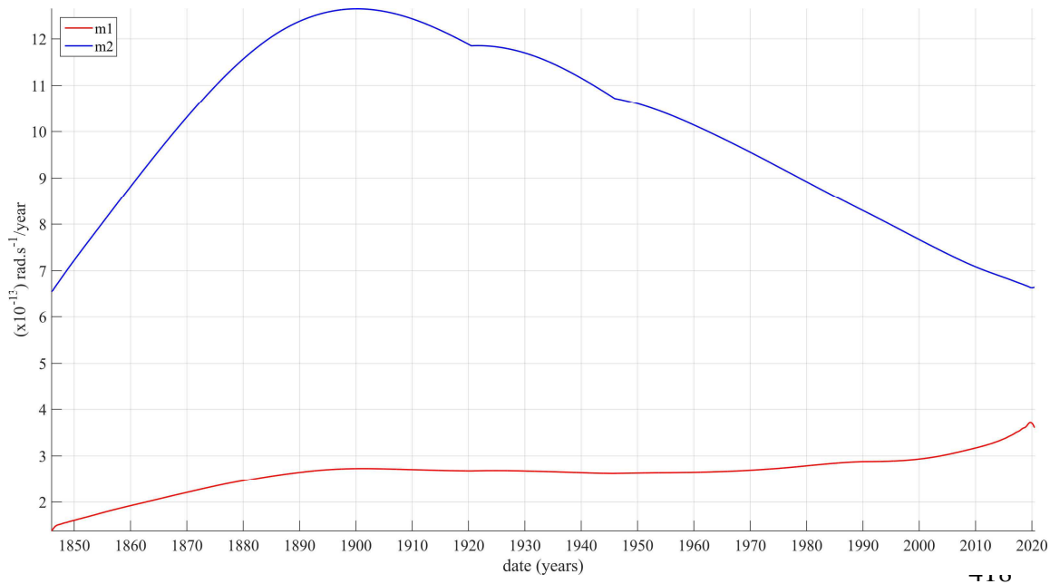
Figure 8a: First SSA component (trend) of the derivative of the Markowitz drift (first SSA component of polar motion). Component m_1 in red and m_2 in blue.
