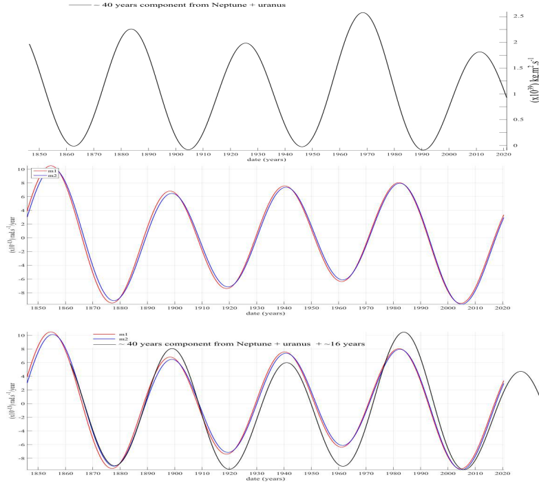
Figure 11b: Superposition (bottom) of the 40yr SSA (first) component of the curve shown in Figure 11a (top) and the component of polar motion with similar pseudo period in Figure 10b (middle). The top curve has been shifted by 16 yr with respect to the middle one in the bottom comparison.
