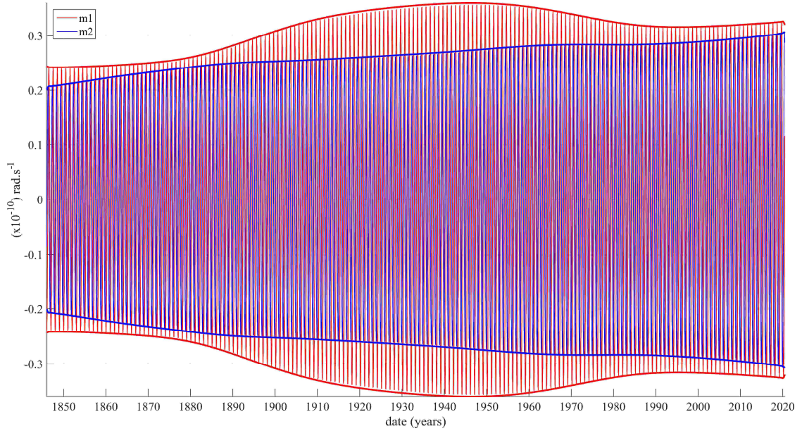
Figure 5: 2nd SSA comp. of polar motion (annual oscillation) since 1846. ( m_1 red, m_2 blue).
