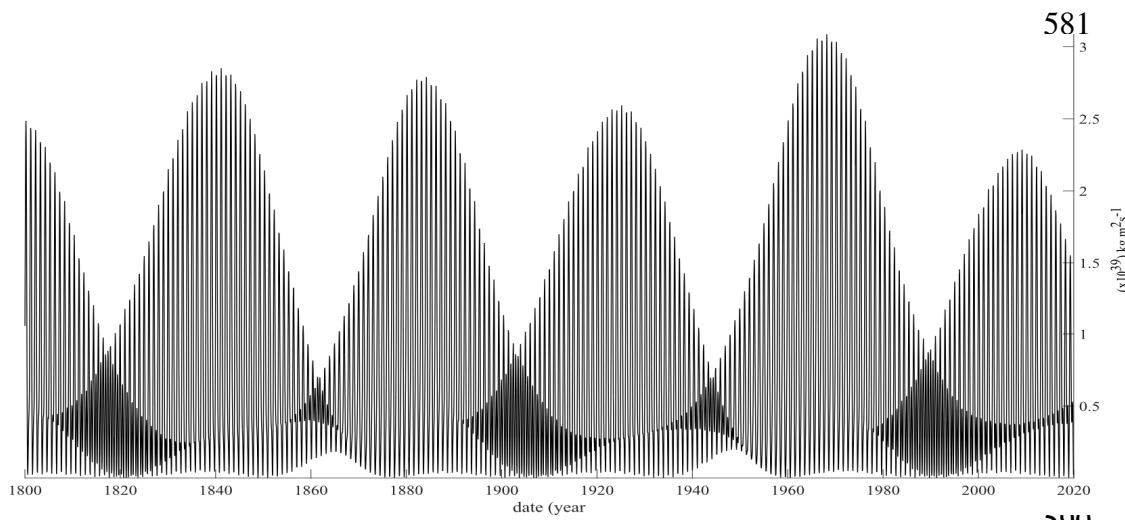
Figure 11a: The sum of the kinetic moments of Uranus and Neptune in a geocentric reference frame.
