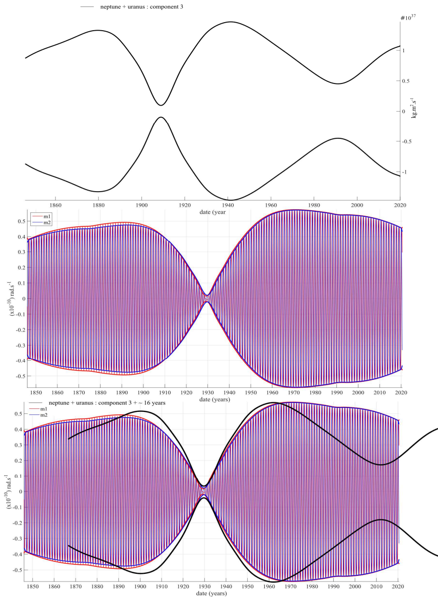
Figure 11d: Third SSA component of the Uranus-Neptune couple (top), Chandler oscillation (third SSA component of polar motion; middle) and comparison of the two with a 16 yr offset.
