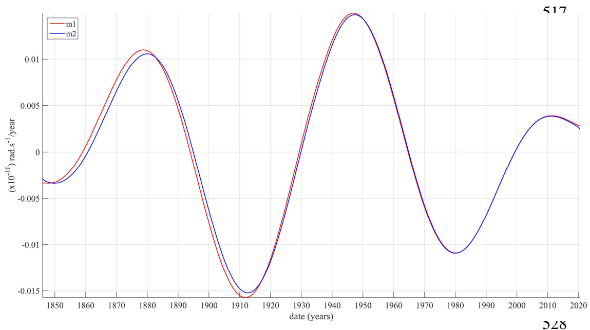
Figure 10a: First SSA component (70 yr quasi-period) of the derivative of the envelope of the Chandler oscillation.
