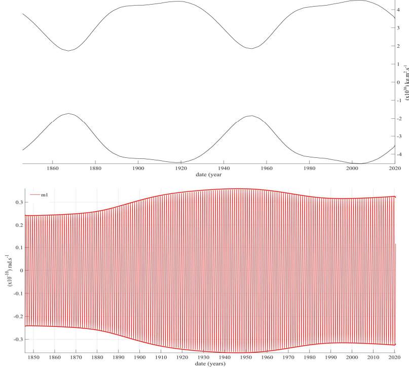
Figure 11c: Second component of the Uranus-Neptune pair (top) and forced annual oscillation of the polar motion m_1 (bottom).
