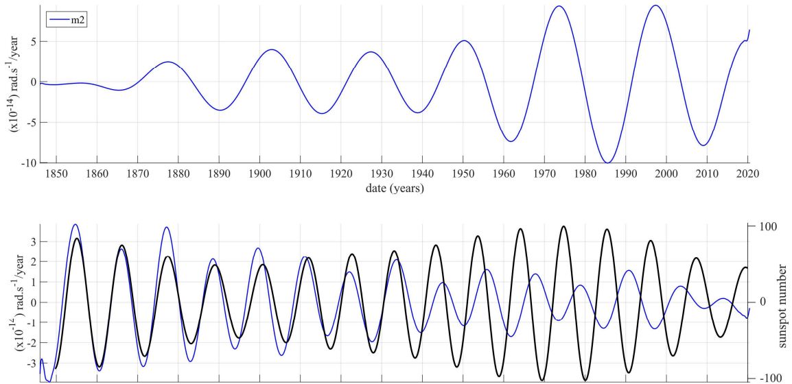
Figure 8d: 22 yr SSA component (top, component m_2 in blue) and 11 yr SSA component (bottom, component m_2 in blue) of the derivative of the Markowitz drift (first SSA component of polar motion). Bottom, black curve: the 11 yr Schwabe cycle extracted by SSA from the sunspot series (sign reversed).
