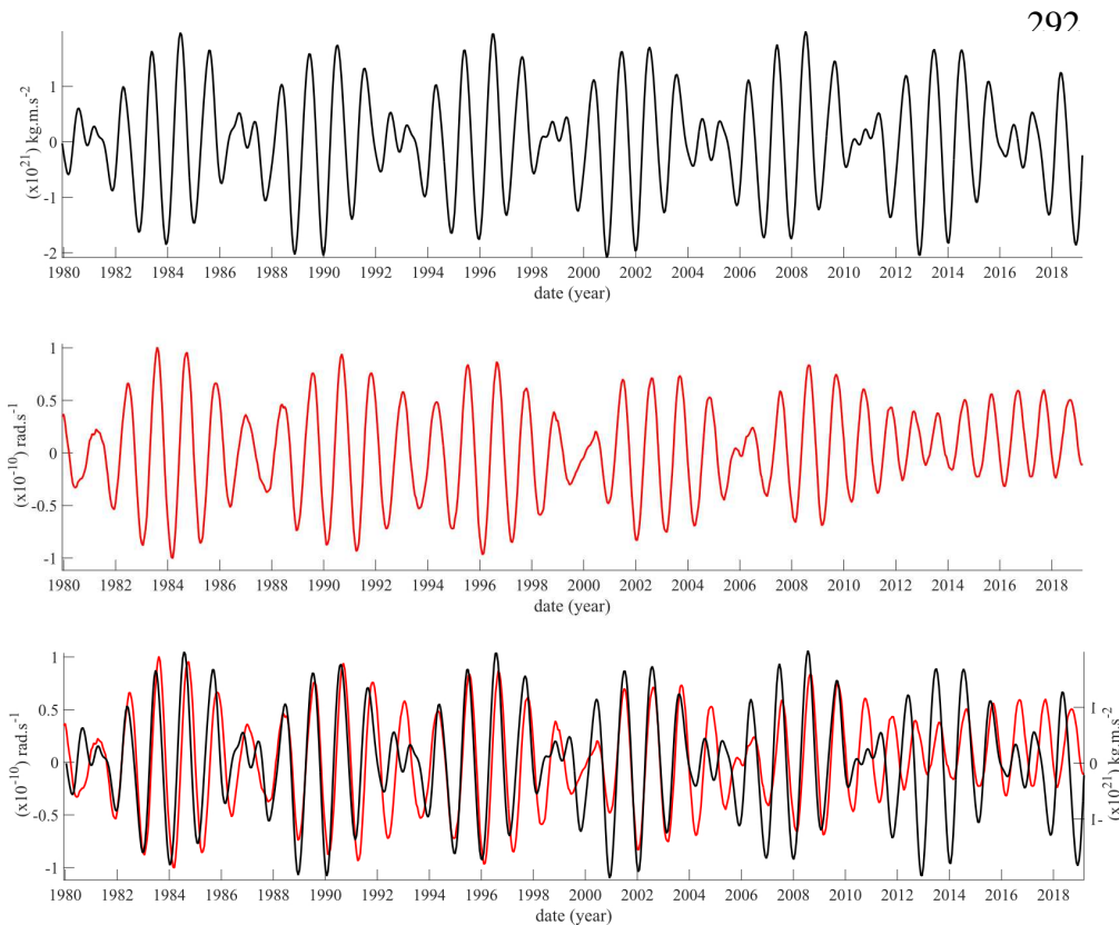
307 Figure 3b: Enlargement of Figure 3a (1980-2019) and superposition of the 2 curves. 308
