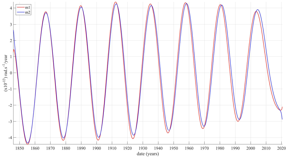
Figure 10d: Fourth SSA component (22 yr quasi-period) of the derivative of the envelope of the Chandler oscillation
