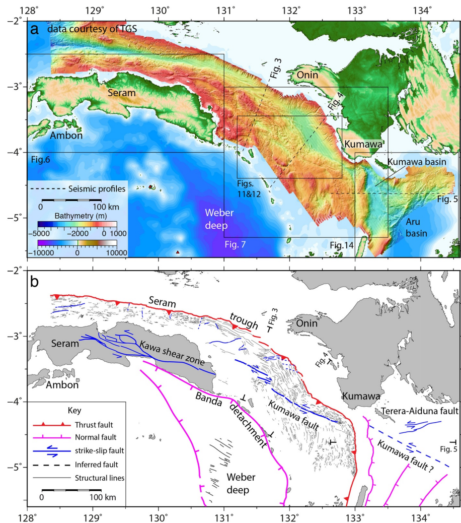
Figure 2. Detailed structural mapping on the east Banda margin using high-resolution bathymetry and topography. (a) A combination of 25-m resolution and 100-m resolution bathymetry showing the base map. (b) Result of structural mapping. For location of the map see Figure 1b.
