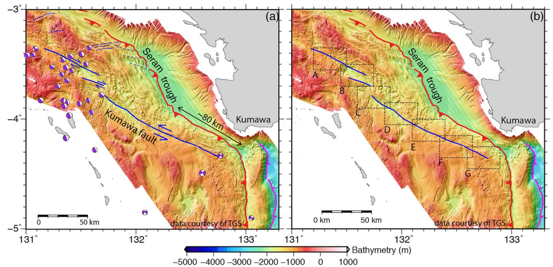
Figure 7. Mapping of the Kumawa fault on high-resolution bathymetry. (a) Mapped structures and earthquakes on bathymetry; note the 80 km displacement on the Seram trough caused by the Kumawa fault and a unique strike-slip earthquake at the SE extremity of the fault. (b) Bathymetry map showing the Kumawa fault, frontal thrust, location of selected regions A-G and bathymetry profiles for detailed structural and morphological analysis.
