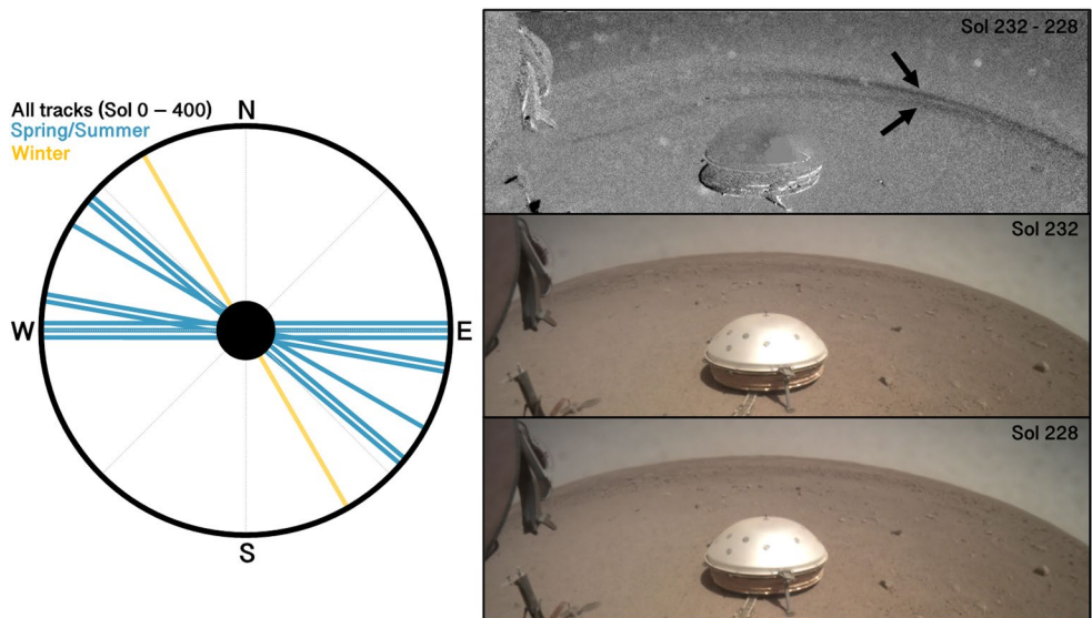
Figure 5. Left: orientation of all dust devil tracks observed in ICC images between Sol 0 and 400. Tracks are primarily oriented NW-SE, consistent with those seen from orbit (Reiss & Lorenz, 2016; Perrin et al., 2020, this issue) and seasonally reversing winds (Banfield et al., 2020). Tracks formed in the winter are driven by dominant northwesterly winds (yellow), and spring and summer tracks are driven by southeasterly winds (blue). The uncertainty in track azimuth angle increases with increasing distance from lander (see Table S1 for track distances). Right: Example of ICC image differencing method for track detection. ICC, Instrument Context Camera.
