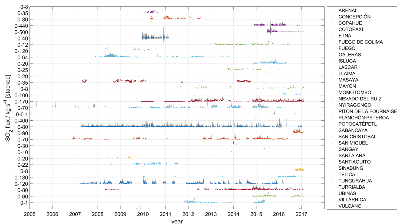
Figure 3. Time series of SO 2 flux for 32 volcanoes in NOVAC from 1 March 2005 to 31 January 2017. Each dot (using a different colour for each volcano) represents the mean of all valid flux measurements obtained in the same day. The grey bars behind the dots represent the 25 %–75 % range of variability in flux for each day. The time series are presented as stacked plots with different scales for the flux, indicated as a range, to better represent the large range of variation between different volcanoes.
