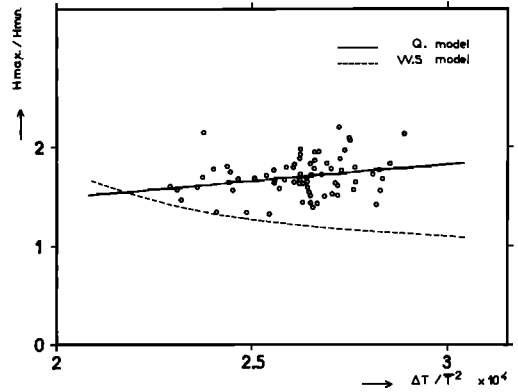
Fig. 20. Comparison of the density ratio H_{\max}/H_{\min} for 1969 orbits with a sun-orbit angle <25^\circ with the theoretical relation found by Quessette [1972] for the exobase distribution controlled by the zero net ballistic flux condition and with the ratio calculated by Wallace and Strobel [1972] in a time-dependent thermospheric model.
