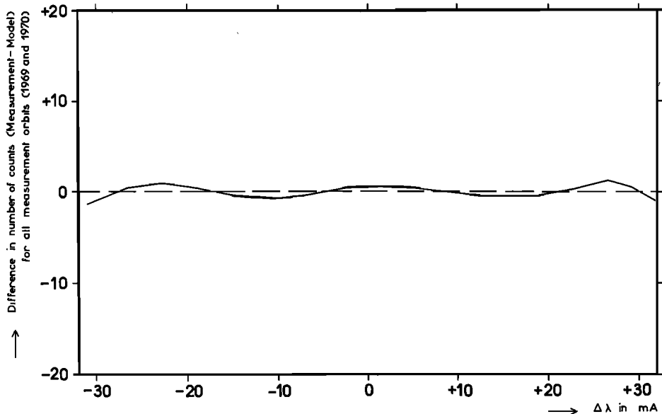
Fig. 17. Deviation from the perfect fit of the best aspherical exospheric model (flat and sloping solar center); all orbits are considered here. Direction of the geocoronal symmetry axis is 1600; T_{max} = 1.3 T_{min} .
