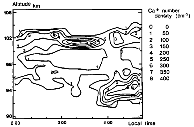
Fig. 3. Calcium ion isodensity contours as a function of local time and altitude (on July, 19, 1983, from 2:00 a.m. to 4:40 a.m.). The density scale is stated in \text{cm}^{-3} on the right side of the figure.
