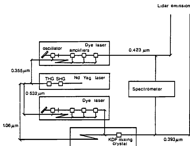
Fig. 1. Schematic configuration of the Yag-Dye system used to generate the 423 nm and 393 nm wavelengths for resonant excitations of Ca and \text{Ca}^+ .
