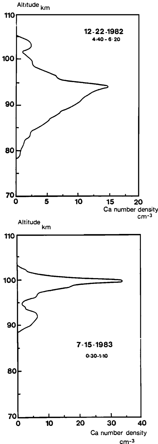
Fig. 2. Calcium atom height profiles obtained by Lidar at the Observatoire de Haute-Provence : a) on December 21/22, 1982, averaged from 4:40 a.m. to 6:20 a.m. b) on July 14/15, 1983, averaged from 0:30 a.m. to 1:10 a.m.
