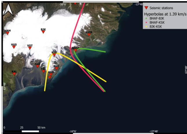
Figure 6: Map showing three hyperbolas for stations BHAF, BJK and KSK for a propagation velocity of 1.39 \text{ km s}^{-1} . Lag times are: 36.65 s for BHAF-BJK, 12.2 s for BHAF-KSK, and –22.65 s for BJK-KSK.
