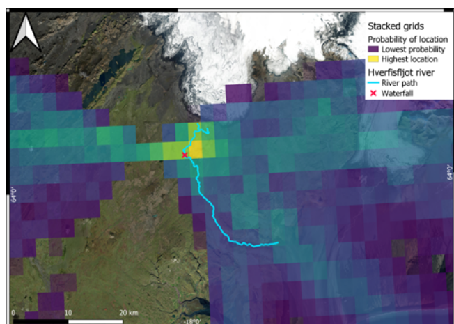
Figure 9: Map showing the stacked probabilities of location at 2.79 \text{ km s}^{-1} for the seasonal source as well as the path of the Hverfisfljót river and the associated waterfall.
