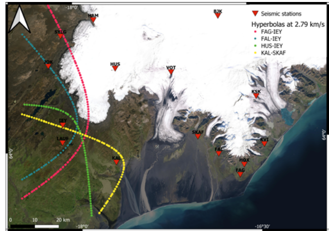
Figure 7: Map showing four hyperbolas for stations FAG, FAL, HUS, IEY, KAL and SKAF for a propagation velocity of 2.79 \text{ km s}^{-1} . Lag times are: –20.05 s for FAG-IEY, –19.3 s for FAL-IEY, –8 s for HUS-IEY, and 10.55 s for KAL-SKAF.
