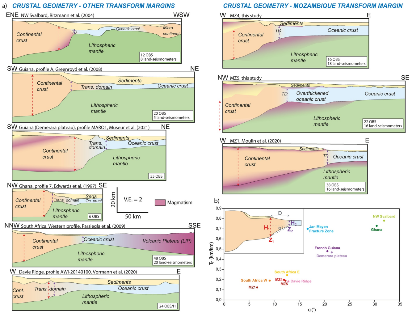
Figure 12. Comparison of the crustal structures of the Mozambique transform margin with other known transform margins. (a) Simplified crustal structures across NW Svalbard, Guiana, Ghana, and South Africa transform margins (Edwards et al., 1997; Greenroyd et al., 2008; Museur et al., 2021; Parsieglia et al., 2009; Ritzmann et al., 2004; Vormann et al., 2020) compared with the structures observed along the sections from the Mozambique transform margin (Moulin et al., 2020; this study). The red and purple arrow refer to the measurements used in Table 4 and panel (b). (b) Diagram showing T_r (crustal thinning ratio, i.e., vertical km for each horizontal km) as a function of \alpha (dip of the Moho), both corrected for the angle of the profile with the trend of the considered transform. Details of how these values were calculated are presented in Table 4.
