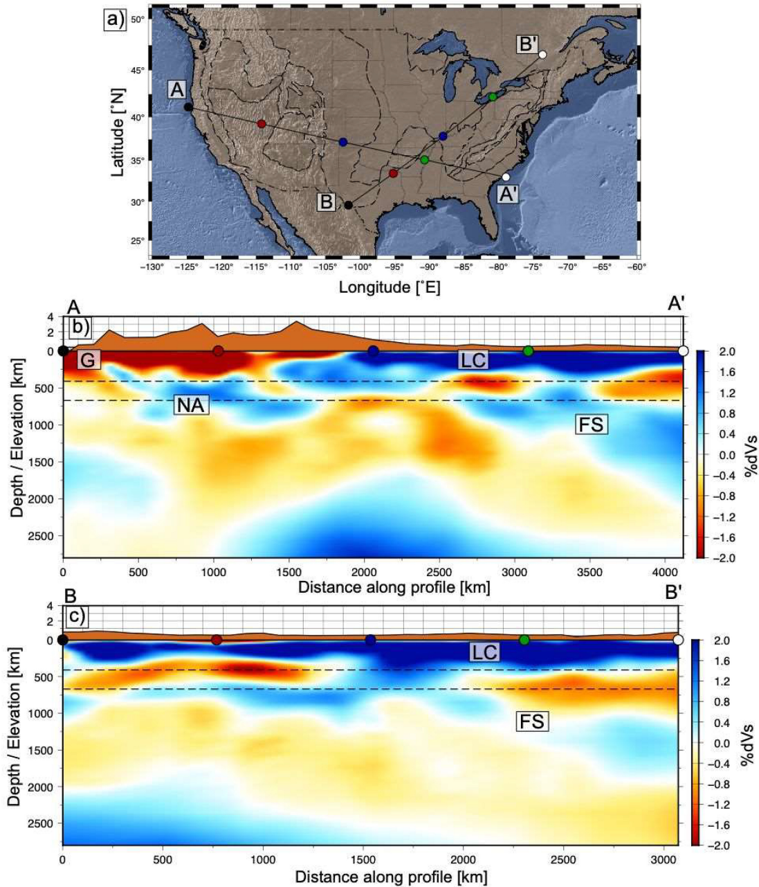
Figure 7. Cross sections along strike and dip of the Farallon system. Labeled features include the Gorda slab (G), Nevada Anomaly (NA), Laurentia Craton (LC) and Farallon Slab (FS). Dashed black lines indicate the Mantle Transition Zone at 410 and 670 km depth. Vertical exaggeration varies with each section. Panel (a) is the location map for lines A–A' and B–B'. Asymmetrically coloured dots on the lines correspond to the surface projections of the same points on the cross-sections. Panel (b) is roughly along the southern edge of the system and panel (c) is along dip of the centre to eastern portion of the slab.
