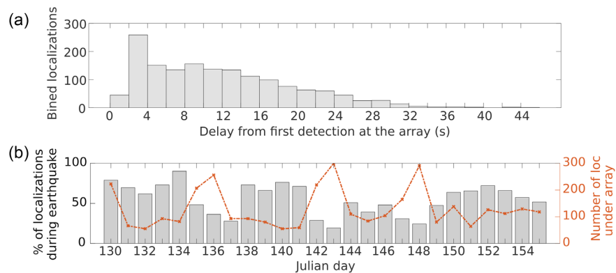
Figure 8. (a) Time delay between observed or estimated first arrival of regional earthquakes and time of MCMC-MFP localization under the array. The first arrival are either picked on borehole data or estimated from the catalogue from Ross et al. (2019). (b) Daily percentage of MCMC-MFP localization during regional earthquakes (grey) and total number of MCMC-MFP localizations under the array (orange).
