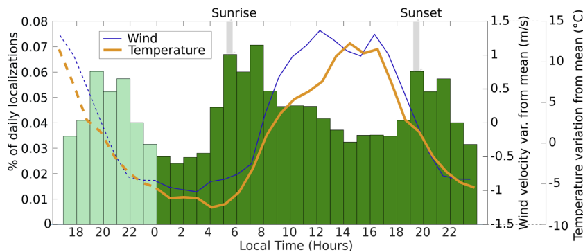
Figure 6. Dark green bars: Average distribution of localizations with backazimuths around 309^\circ and apparent velocities around 3750 \text{ m s}^{-1} , stacked over 24 hr according to local time. Light green bars: duplicate of the stack between 17:00 and 00:00, used to highlight the periodicity. Orange line: Temperature variations relative to the daily mean averaged over 26 d. Dark blue line: Wind gust velocity variations relative to the daily mean averaged over 26 d.
