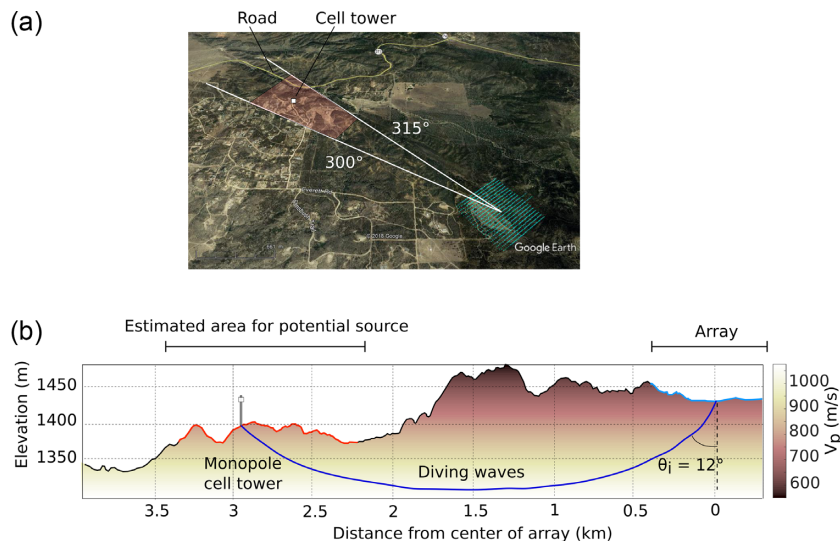
Figure 4. (a) Superposition of the source direction on the Google earth view. The red area correspond to the point of origin for P waves estimated for apparent velocities ranging from 3500 to 5000 \text{m s}^{-1} using the 1-D gradient velocity profile shown Fig. 3(c). (b) Bathymetry along the source direction. The blue area corresponds to the array position. The red area correspond to the point of origin for P waves. The P -wave velocity profile is shown in the background.
