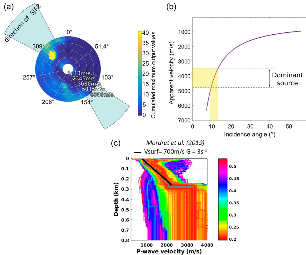
Figure 3. (a) Stacked localizations according to the apparent velocity and backazimuth at 16 Hz, weighted by the value of the maximum output for each localization. The blue cones indicate the direction of the fault. (b) Apparent velocity according to incidence angle computed for an average 1-D gradient velocity model. The yellow area corresponds to the incidence angle and apparent velocities of the dominant source. (c) Background: 1-D velocity model inverted by Mordret et al. (2019). Black line: average 1-D gradient velocity model used for this study.
