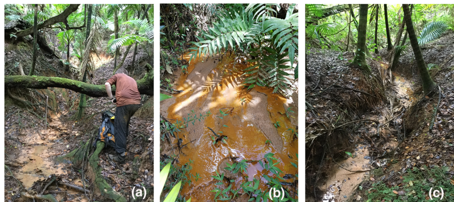
Figure 4. (a) Image of the channel headwall and unchanneled flow from the seep. (b) Seep waters saturate piles of sediment at the base of headwalls where they emerge from the subsurface. (c) Seep waters forming a channel with well-defined banks.
