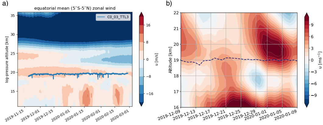
Figure 3. Equatorial zonal winds simulated by ERA5. a) Time-height variations in zonal mean zonal wind averaged between 5°SN and 5°S with the balloon altitude (blue line). The zonal mean zonal wind shows the structure of the QBO above the tropopause. b) Eight-day-running-mean zonal wind along the balloon flight-track as a function of altitude and time. The dark-blue dashed line shows the daily averaged altitude of the balloon.
