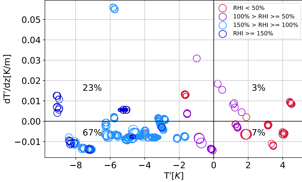
Figure 2. Wave influence on cirrus cloud detections at and around South America. The plot shows the distribution of particles \geq 3\mu\text{m} , considered to be ice, as a function of wave perturbations ( T' ) and the vertical gradient of the temperature perturbation T' ( dT'/dz \sim dT'/dt ). The colors refer to relative humidity above ice (RHI) and the percentages given in the quadrants are the percentage of particles found in the respective quadrant relative to all particle counts. The circle sizes are proportional to particle concentrations where small circles represent 1/liter, medium size circles 3/liter and the largest circles 6/liter.
