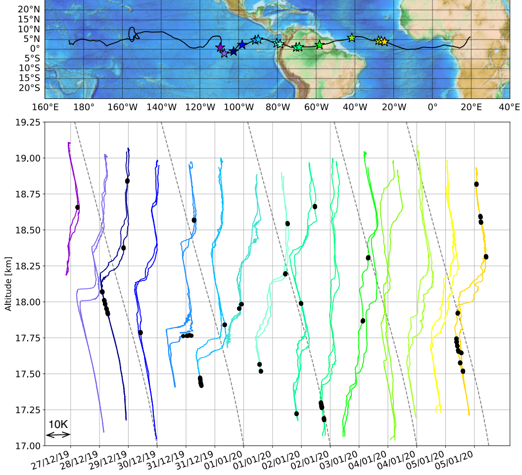
Figure 1. Flight track of the TTL3 balloon during the Strateole-2 campaign from 9th December to 9th January. The stars show the positions of the pairs of descending/ascending RACHuTS temperature perturbation profiles shown in the lower panel. Each pair of RACHuTS profiles are separated by 10K. The color coding corresponds to the location of the profile (see map) and the date of the profile pair is given on the x-axis. The gray vertical lines highlight T' = 0 for each night's pair of profiles. Temperature perturbations are due to waves with periods < 30 days. Black dots represent the location of ice observations and the black dashed lines show the slope of perturbations giving a net adiabatic lapse rate, indicating mixed layers.
