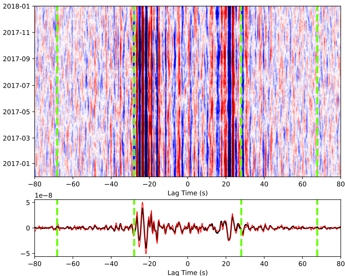
Figure 2. Interferogram plot for the vertical–vertical components of station pair JSP–SJQ with an interstation distance of 56 km. Green dashed bars indicate the coda windows for this station pair. Above: interferogram plot for 30-d stacks for just over 1 yr with red showing positive amplitude and blue showing negative amplitude. Below: waveform of cross-correlations with the black line showing the reference stack and the red line showing the daily cross-correlation on 2016 December 1.
