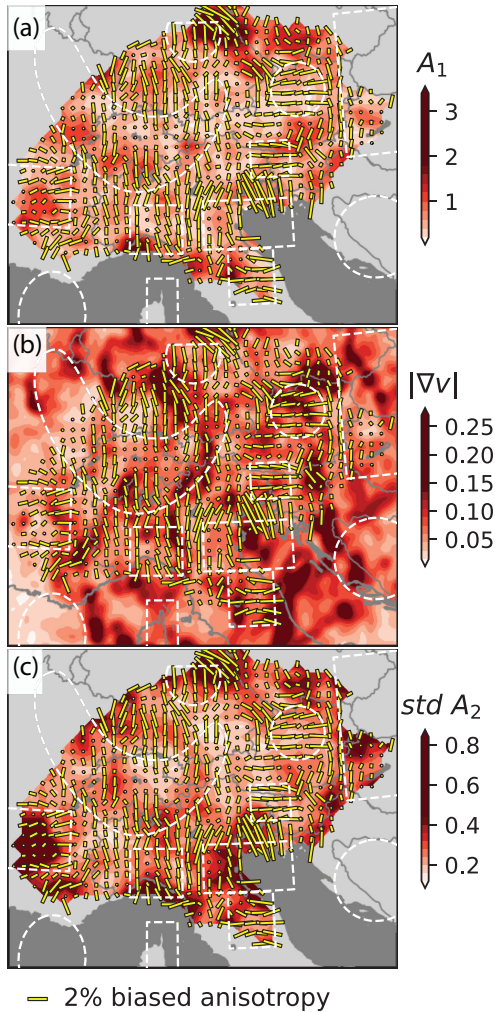
Figure 8. The anisotropic bias presented in Fig. 6 (f) ( \pm 2 per cent isotropic velocity variation) is compared to three different parameters: (a) to the strength of the \Psi_1 anisotropy, (b) to the gradient of the velocity field calculated from the input model and (c) to the standard deviation of A_2 (amplitude of the \Psi_2 anisotropy; its standard deviation can be calculated from the fitting procedure to eq. 2). A weak spatial correlation between the biased anisotropy and the strength of all three chosen parameters can be seen.
