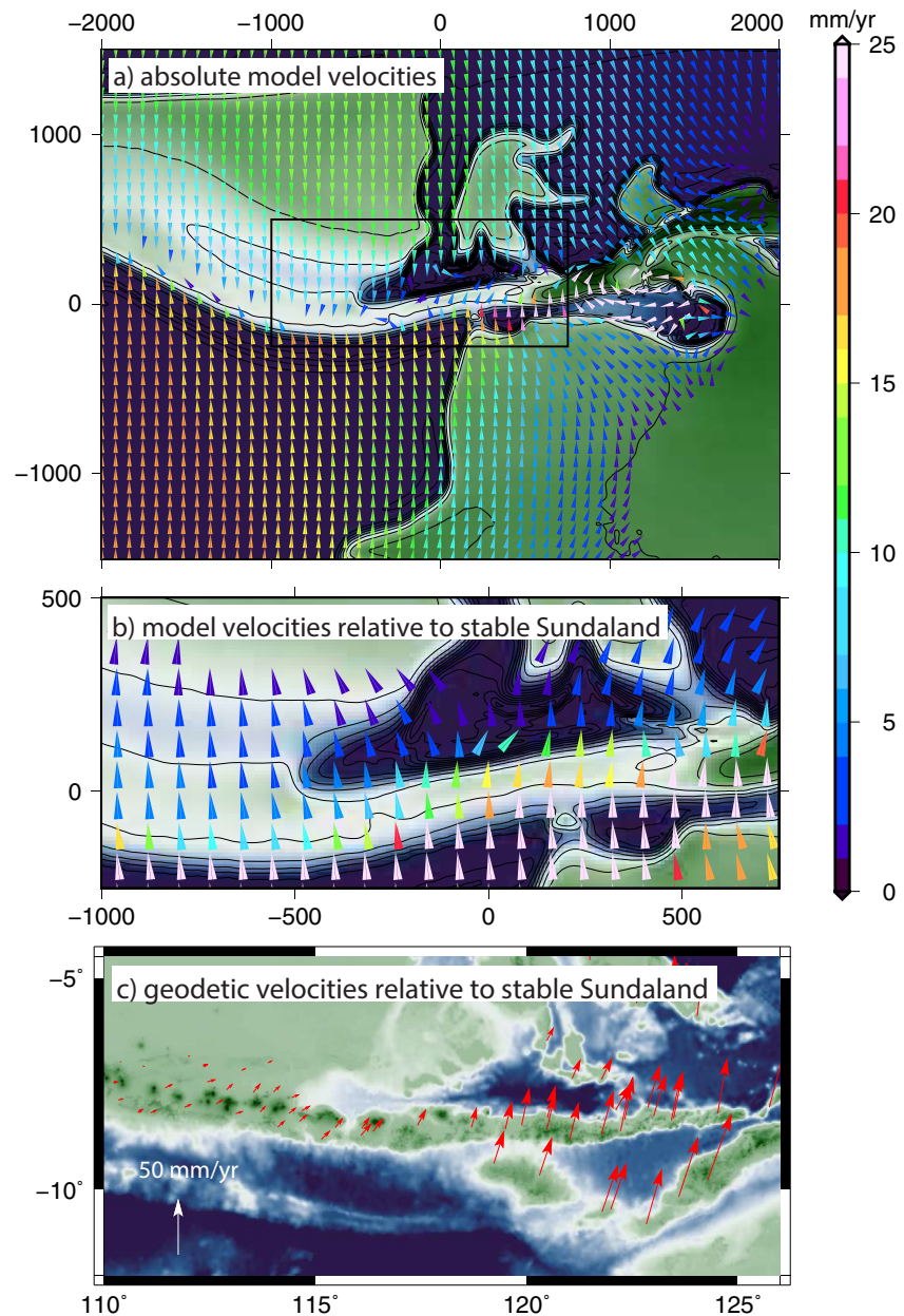
Figure 5. Observed and modeled surface velocities. (a) Global velocities in the model reference frame; (b) zoomed in velocities, with respect to stable Sundaland (at coordinate -500/500 km). (c) Geodetic velocities relative to Sundaland (Koulali et al., 2016) at an approximately comparable geographical scale than in panel (b).
