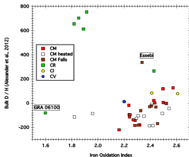
Fig. 7. Comparison between the average oxidation factor of iron with the bulk D/H ratio from Alexander et al. (2012) for the different groups of carbonaceous chondrites. (Color figure can be viewed at wileyonlinelibrary.com .)
