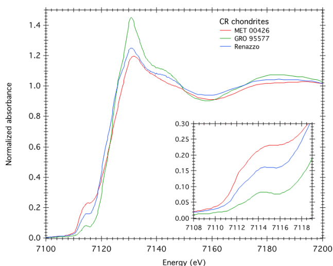
Fig. 2. Normalized XANES spectra of CR chondrites with inset expanded diagram of the pre-edge feature. (Color figure can be viewed at wileyonlinelibrary.com .)
