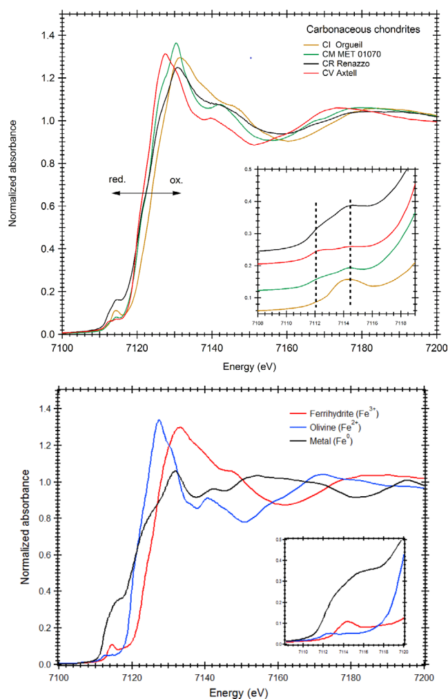
Fig. 1. a) Normalized XANES spectra of selected carbonaceous chondrites with enlarged pre-edge feature. b) XANES spectra references for Fe 0 , Fe 2+ , and Fe 3+ oxidation state. (Color figure can be viewed at wileyonlinelibrary.com .)
