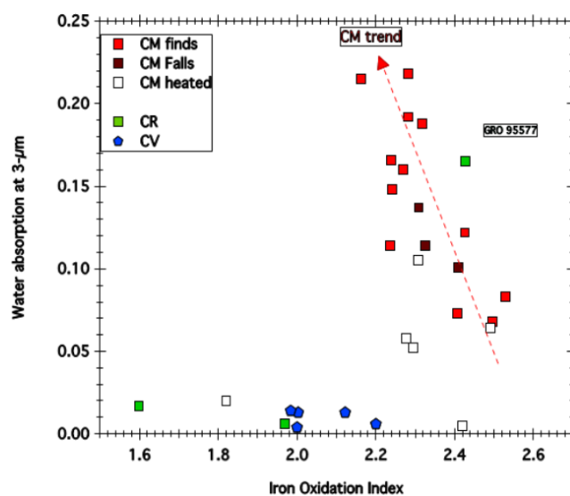
Fig. 6. Comparison between the average oxidation factor of iron with the 3 \mu\text{m} water band from Beck et al. (2014) for the different groups of carbonaceous chondrites. (Color figure can be viewed at wileyonlinelibrary.com .)
