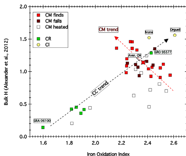
Fig. 5. Comparison between the average oxidation factor of iron bulk H content (from Alexander et al. 2012) for the different groups of carbonaceous chondrites. (Color figure can be viewed at wileyonlinelibrary.com .)
