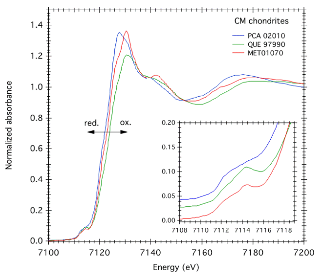
Fig. 3. Normalized XANES spectra of CM chondrites with inset expanded diagram of the pre-edge feature. (Color figure can be viewed at wileyonlinelibrary.com .)
