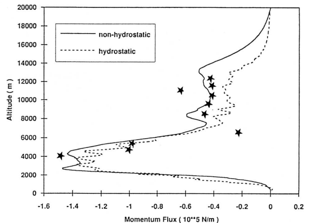
FIG. 9. Flux of momentum measured by the research aircraft on 15 October 1990 and simulated by two versions of the MERCURE model (from Elkhalfi and Carissimo 1993).
