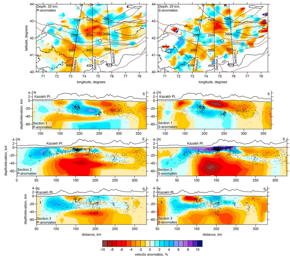
Figure 9. P and S wave velocity anomalies in vertical sections. The locations of the profiles are indicated in the maps in the upper part of the Figure. The projections of events located at distances of less than 40 km from the profile are indicated with black dots. The exaggerated topography along the profiles is shown above each section.
