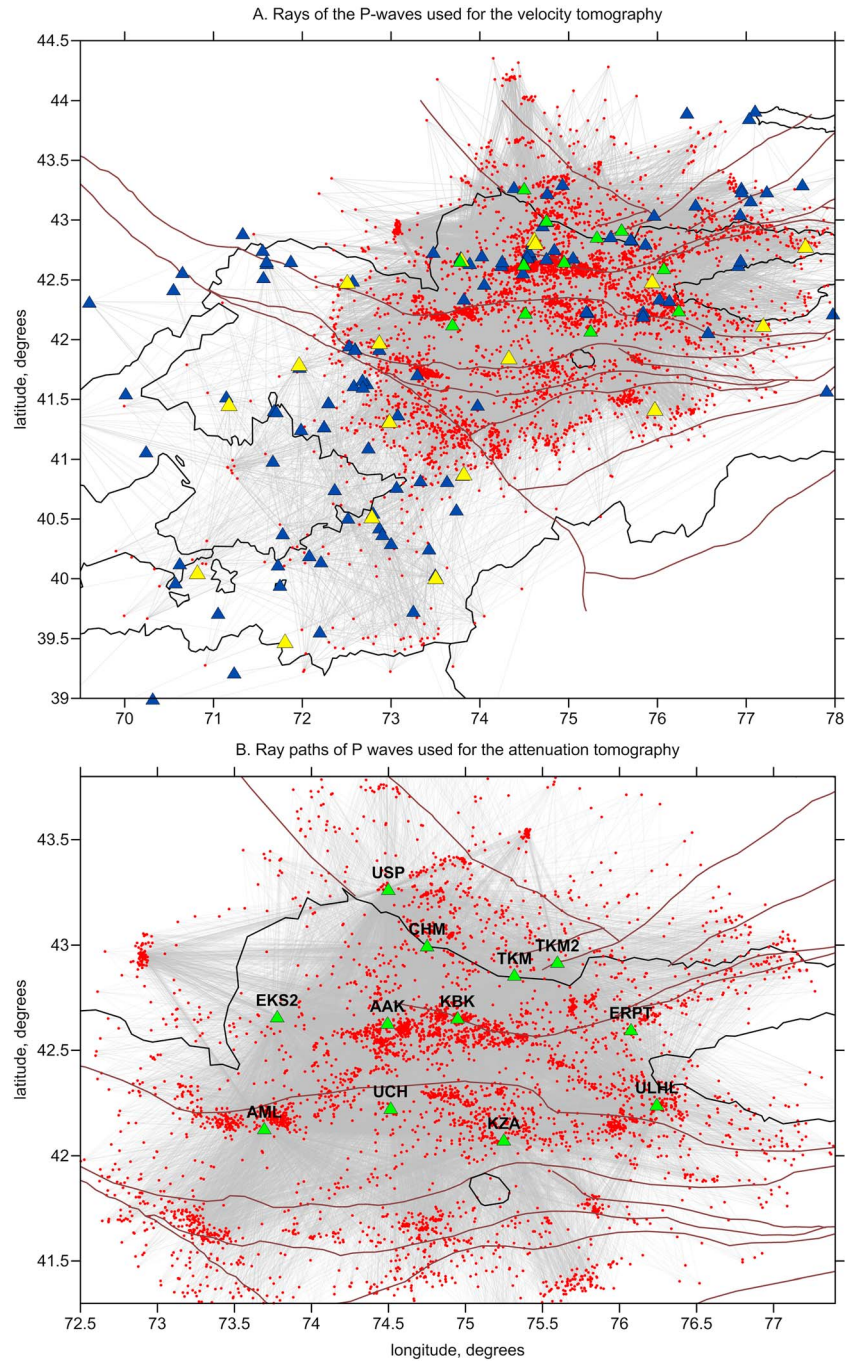
Figure 2. The distributions of data in tomography studies for (a) velocity and (b) attenuation. The green triangle depicts KNET, the yellow triangle depicts KRNET, the blue triangles depict other seismic stations, and the red dots are the earthquakes. The grey lines represent the paths of the P rays. For the S wave data, the ray configurations are similar. In b, the violet lines represents the major faults.
