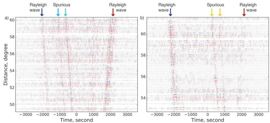
Figure 4. Correlation functions computed between a subnetwork and a distant, trans-Atlantic station filtered for the period band 15 s to 25 s. For the sake of clarity, the signals are averaged in 0.15^\circ distance bins. (a) Correlations between station BFO in Europe and the subnetwork in the U.S. (b) Correlations between I57A in the U.S. and the subnetwork in Europe.
