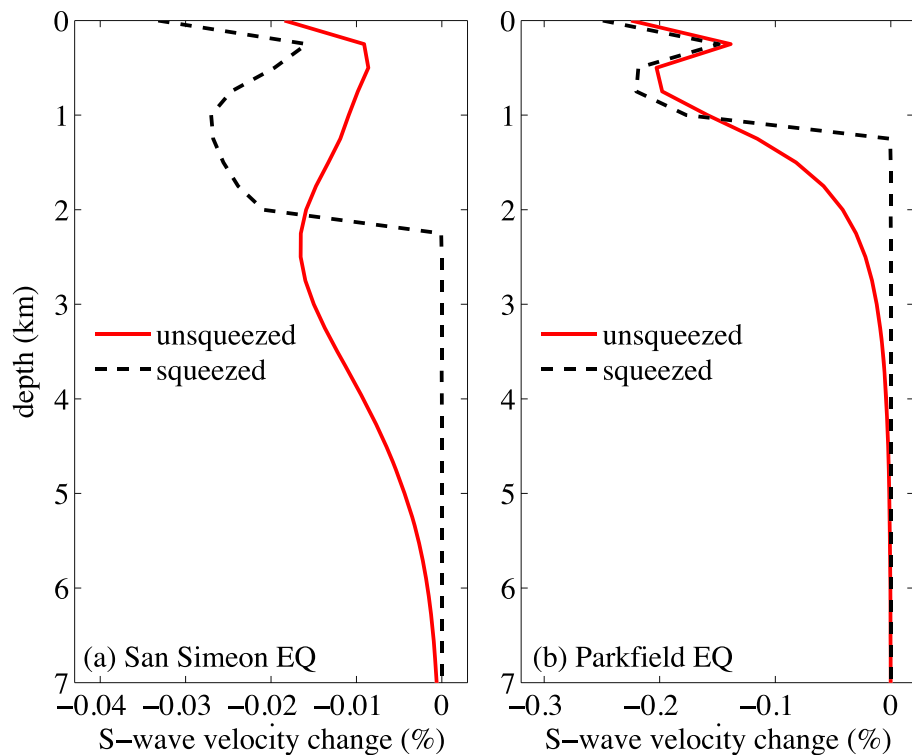
Figure 5. Inverted S wave velocity changes in percentage at difference depths. The red solid curve shows the unsqueezed solution, and the black dashed curve shows the squeezed solution for (a) the San Simeon earthquake and (b) the Parkfield earthquake.
