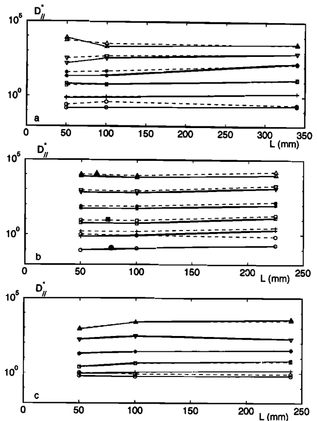
Figure 11. Dispersion coefficients D_{||t}^* (solid), D_{||a}^* (dashed) and D_{||s}^* (solid symbols) for a flow along the (a) x , (b) y , and (c) z directions versus the sampling distance from the inlet L (for D_{||t}^* and D_{||a}^* ) or the instantaneous mean displacement \langle L_i \rangle (for D_{||s}^* ). Data are for Pe_n = 0.01 (circles), 0.1 (crosses), 1 (squares), 10 (stars), 100 (inverted triangles), and 1000 (triangles).
