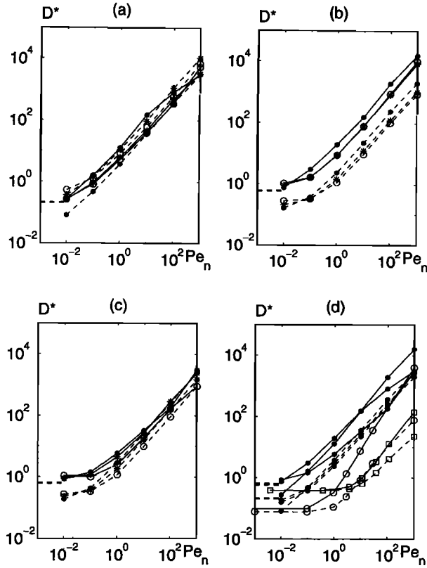
Figure 12. Dispersion D_{\parallel a}^* (solid lines) and D_{\perp a}^* (dashed lines) as functions of the Péclet number for a pressure direction along the (a) x direction, (b) y direction, and (c) z direction, measured at distances L_1 (open circles), L_2 (stars), and L_3 (solid circles) from the inlet. The horizontal lines are the predictions of D_{\parallel}^* from equations (34a) and (35) for vanishing Pe_n . The results for L_3 (solid circles) for the three flow directions are compared in Figure 12d to the data of O. Huseby et al. (manuscript in preparation, 2000) for isotropic networks of hexagonal fractures with density \rho' = 4 (open circles) and 12 (squares).
