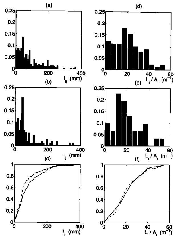
Figure 5. Histograms (a and b) of the intersection lengths l_{ij} , in millimeters and (d and e) of the total intersection length per fracture and per unit area L_i/A_i , in \text{m}/\text{m}^2 . Figures 5a and 5d are relative to all the fractures in the network, while the fractures which intersect the lateral boundaries of the sample are removed in Figures 5b and 5e. (c and f) The cumulated distribution functions corresponding to Figures 5a and 5b and to Figures 5d and 5e, respectively. The solid (dashed) line corresponds to the complete (filtered) network.
