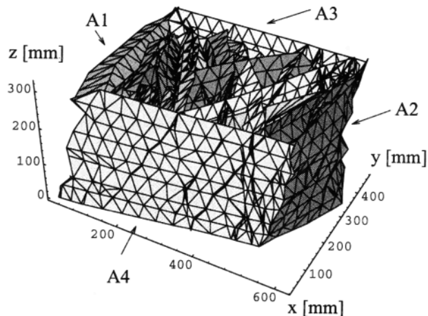
Figure 7. Artificial fractures A1-A4 which surround the sample volume, used to impose the hydraulic boundary conditions. Graduations are in millimeters.
