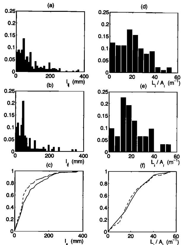
Figure 5. Histograms (a and b) of the intersection lengths l_{ij} , in millimeters and (d and e) of the total intersection length per fracture and per unit area L_i/A_i , in m/m^2 . Figures 5a and 5d are relative to all the fractures in the network, while the fractures which intersect the lateral boundaries of the sample are removed in Figures 5b and 5e. (c and f) The cumulated distribution functions corresponding to Figures 5a and 5b and to Figures 5d and 5e, respectively. The solid (dashed) line corresponds to the complete (filtered) network.
