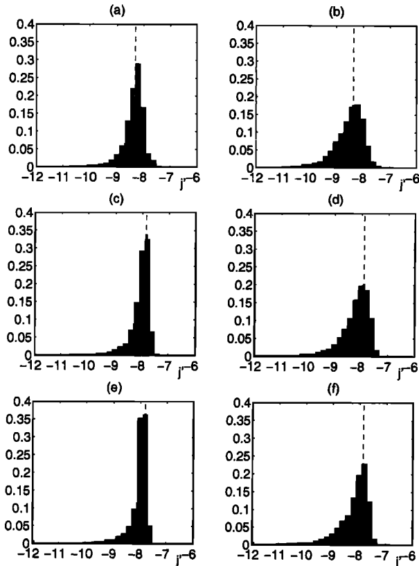
Figure 9. Histograms of the decimal logarithm of the flow rate j' in the triangles for a mean flow direction along the (a and b) x axis, (c and d) y axis, and (e and f) z axis. The histograms are weighted by the triangle areas. The local permeabilities are all equal to \sigma_0 in Figures 9a, 9c, and 9e; they are uniformly distributed between 0 and 2\sigma_0 in Figures 9b, 9d, and 9f. The vertical dashed line is the surface average corresponding to the global flux.
