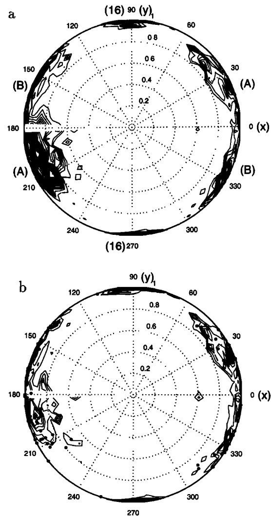
Figure 3. Distributions of the unit vectors normal to the triangles, (a) in numbers and (b) weighted by the areas, in projection onto the ( x , y ) plane. The origin of the azimuthal angle is aligned with the x axis. Families A and B and fracture 16 are marked in Figure 3a. The solid dots in Figure 3b correspond to the surface-averaged normal vectors of the whole fractures.
