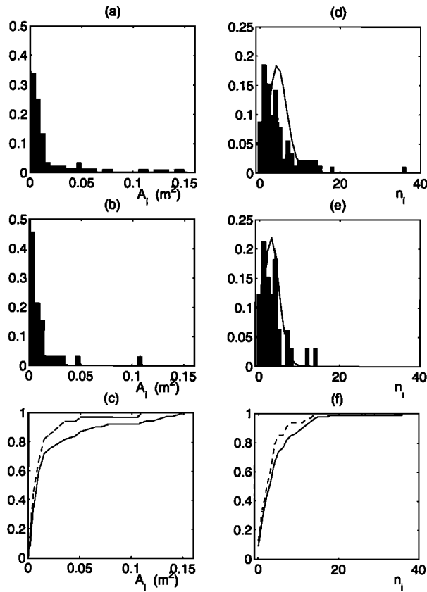
Figure 4. Histograms (a and b) of the fracture surface areas A_i , in \text{m}^2 and (d and e) of the number n_i of intersections per fracture. Figures 4a and 4d are relative to all the fractures in the network, while the fractures which intersect the lateral boundaries of the sample are removed in Figures 4b and 4c. The solid line in (d,e) is the Poisson distribution with the same average. (c and f) The cumulated distribution functions corresponding to Figures 4a and 4b and to Figures 4d and 4e, respectively. The solid (dashed) line corresponds to the complete (filtered) network.
