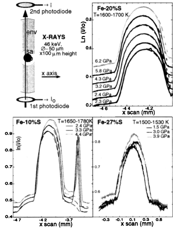
Figure 3. Absorption scans for liquid Fe- x\% S (for the Fe-27%S experiment, the energy was fixed to 58 keV) and sketch of the scan geometry through the cell-assembly (upper left). Dashed lines are fits of the data; subscripts liq , env and sa stand for liquid, sample environment and sapphire; the peak at x \sim -3.55 mm (lower left) corresponds to the Pt microfoil used for internal P-T calibration.
