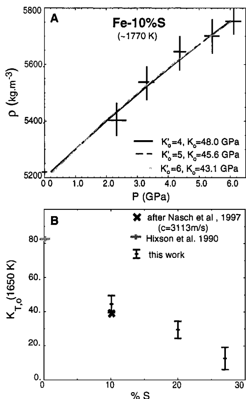
Figure 4. A - Density as a function of pressure for the Fe-10%S experiment; B - bulk incompressibility, K_T , as a function of the wt% S content. For convenient comparison, the plotted K_T values all correspond to the same 1650 K isotherm; error bars on K_T include tests for a 4-7 K'_o range as well as uncertainties on density measurements.
