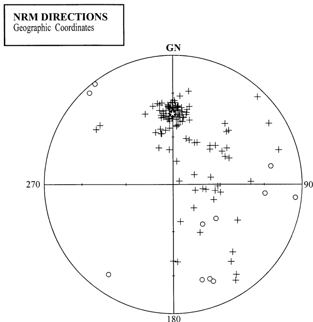
Figure 4. Equal-area plot of the NRM directions for all samples (crosses: positive inclinations; open circles: negative inclinations). Open star: present magnetic field direction.
