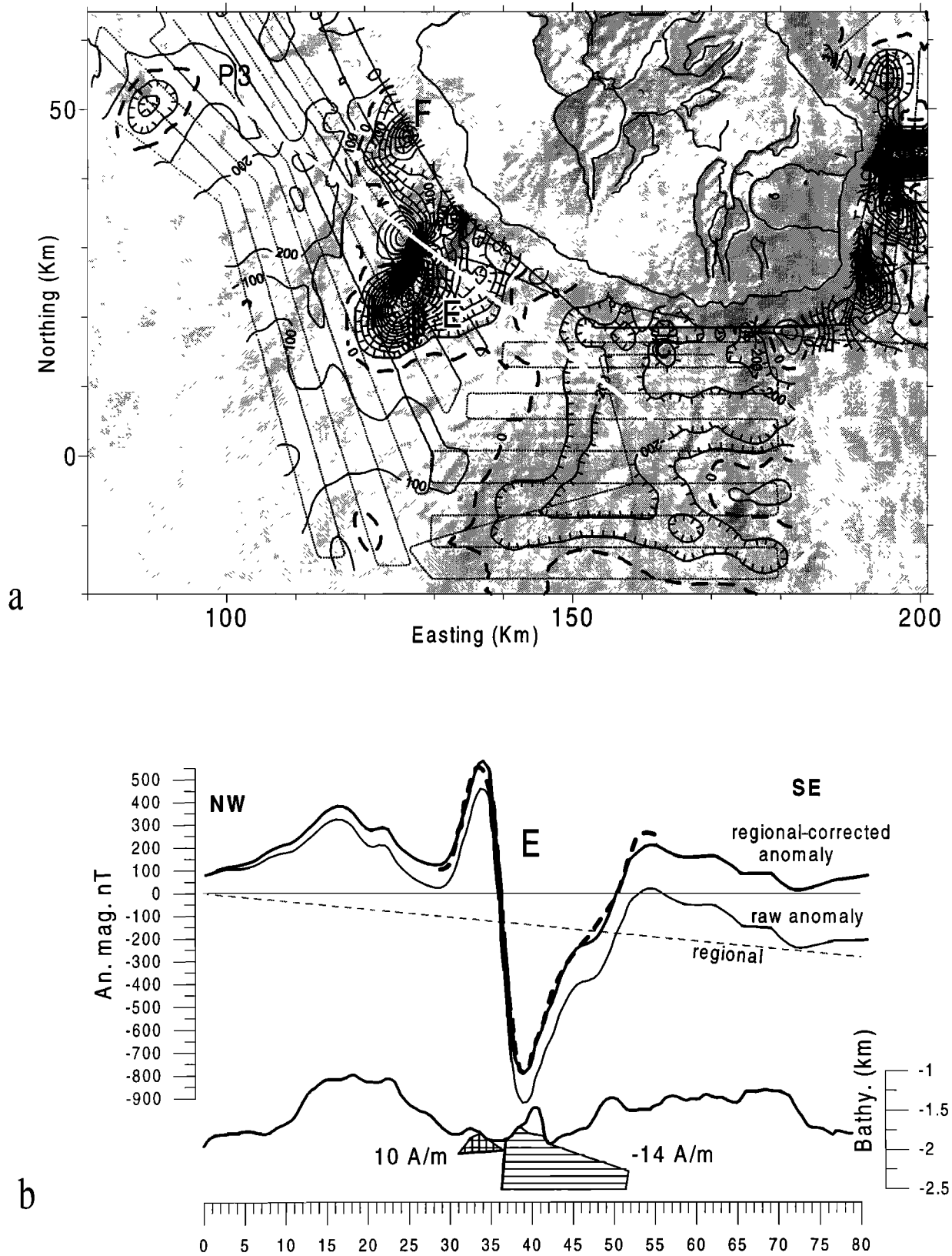
Figure 5. Interpretation of the RTP sea level magnetic anomaly near the southwestern seashore. (a) Anomaly map superimposed on shaded bathymetry. E and F are anomalies discussed in the text. P3 is the line of profile for Figure 5b. Magnetic contours are 100 nT. Black dots show location of the magnetic measurements along the ship track. (b) Bathymetric and magnetic profiles of anomaly E along line P3; dashed line, 2-D model profile.
