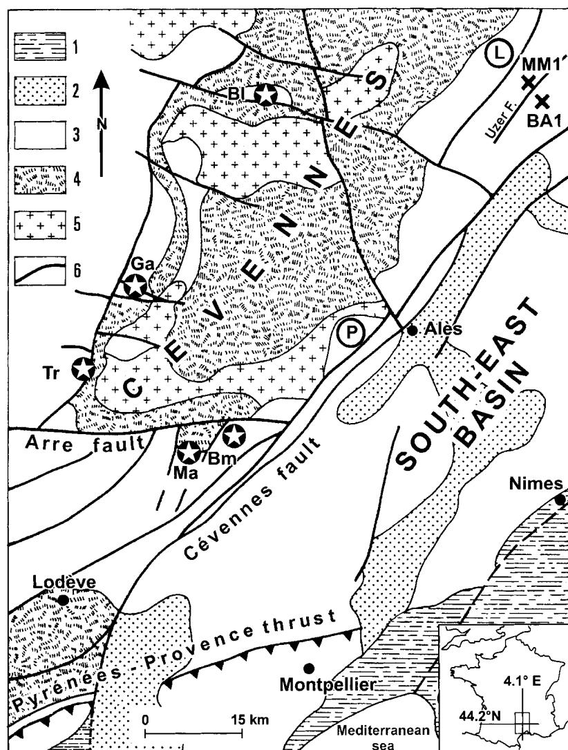
Figure 1. Structural map and locations of sampling sites. 1–Quaternary; 2–Oligo-Miocene; 3–Mesozoic to Eocene; 4–Palaeozoic; 5–Late Hercynian granites; 6–faults. Studied areas: L–Largentière; P–La Croix-de-Pallières. Boreholes GPF: MM1–Morte Mérie; BA1–Balazuc. Named ore deposits: Ma–Les Malines; Bm–Bois-Madame; Tr–Trèves; Ga–Gatuzières; BL–Le Bleyard.
