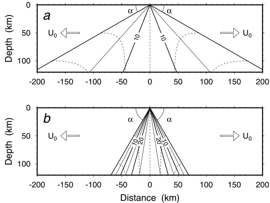
Figure 13. Corner flow solutions showing contours of vertical component of velocity (solid lines; contour interval is 5 \text{ mm yr}^{-1} ) and mantle matrix streamlines (dashed lines) calculated from Equations (1) and (2). (a) Wedge angle \alpha = 30^\circ , plate half spreading rate U_0 = 10 \text{ mm yr}^{-1} . (b) \alpha = 60^\circ , U_0 = 10 \text{ mm yr}^{-1} .
