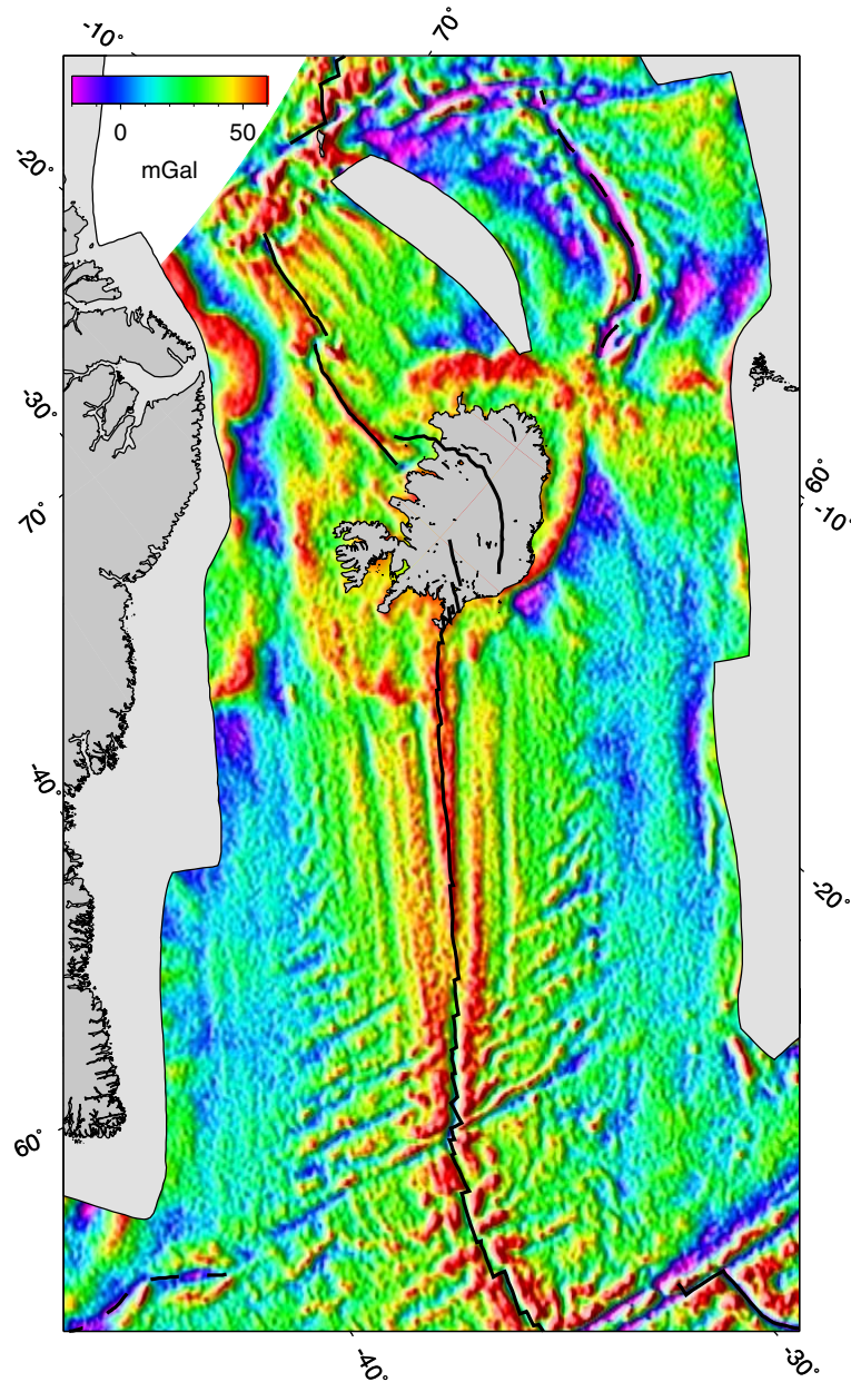
Figure 2. Free-air gravity field around Iceland from satellite altimetry, illuminated from the north-west [ Sandwell and Smith, 1997 ].
