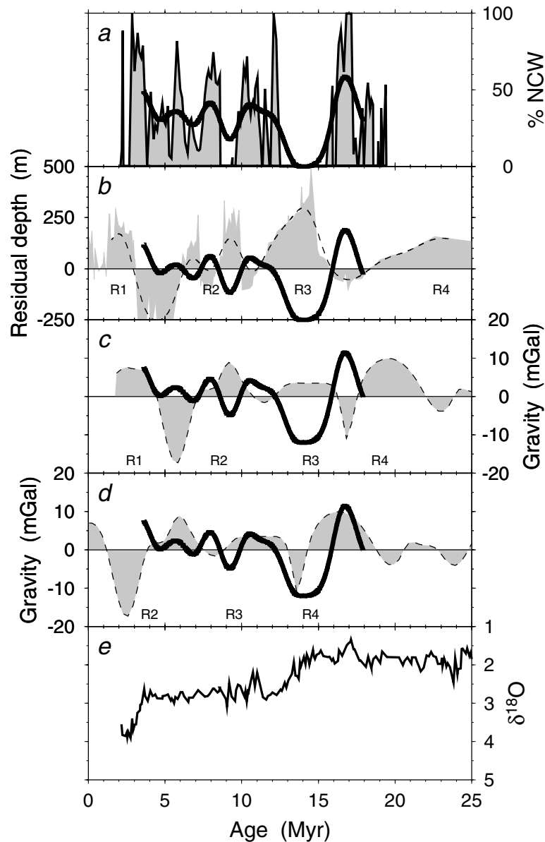
Figure 12. (a) Record of Northern Component Water flux estimated by recording benthic foraminiferal \delta^{13}\text{C} changes in the Southern Ocean relative to changes in the North Atlantic and Pacific records, from Wright and Miller [1996]. Thick black line shows this record filtered at a wavelength of 3 Myr; this filtered record is also superimposed on plots (b), (c) and (d). (b) V-shaped ridge record of Wright and Miller [1996] (grey shading), based on anomalous topography observed on a seismic transect perpendicular to the Reykjanes Ridge, shifted in time so that peaks correspond to times that melting anomalies were situated beneath Iceland. Dashed line shows this record filtered at a wavelength of 3 Myr. (c) V-shaped ridge record from short-wavelength gravity field of the Irminger Basin (Figure 10) (grey shading, dashed line), with a time shift of +1.5 Myr so that peaks correspond to times that melting anomalies were situated beneath Iceland. This time shift is calculated by noting that the gravity record is from crust formed 300 km from Iceland, and that the V-shaped ridges propagate at around 200 km Myr. (d) Same as plot (c) but with a time shift of -1.75 Myr, equivalent to the anticipated record of uplift 650 km from Iceland. (e) Benthic foraminiferal \delta^{18}\text{O} curve of Wright and Miller [1996]. The middle Miocene \delta^{18}\text{O} increase and development of northern hemisphere glaciation during the Pliocene correspond to ridges R1 and R3 respectively, and to changes in flux of Northern Component Water. This match may suggest a link between V-shaped ridges and climate change.
