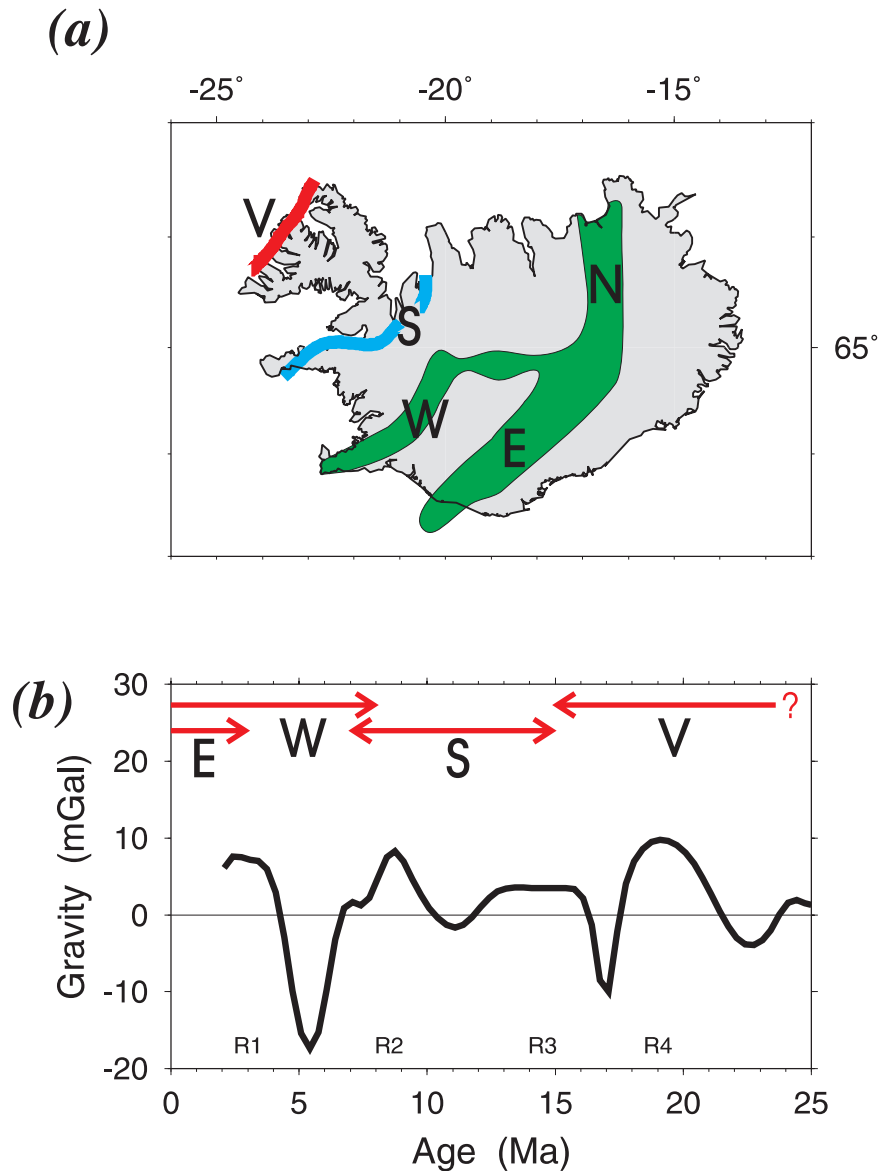
Figure 14. Relationship between gravity record of V-shaped ridges and spreading axis jumps onshore Iceland. (a) Location of active and extinct spreading axes on Iceland. E = Eastern Volcanic Zone; N = Northern Volcanic Zone; S = Snaefellsnes paleo-rift axis; V = Vestfirðir paleo-rift axis; W = Western Volcanic Zone. (b) Black line is the V-shaped ridge record from the short-wavelength gravity field of the Irminger Basin (Figure 10), with a time shift of +1.5 Myr so that peaks correspond to times that melting anomalies were situated beneath Iceland. Red arrows mark times each spreading axis has been active, after Hardarson et al. [1997].
