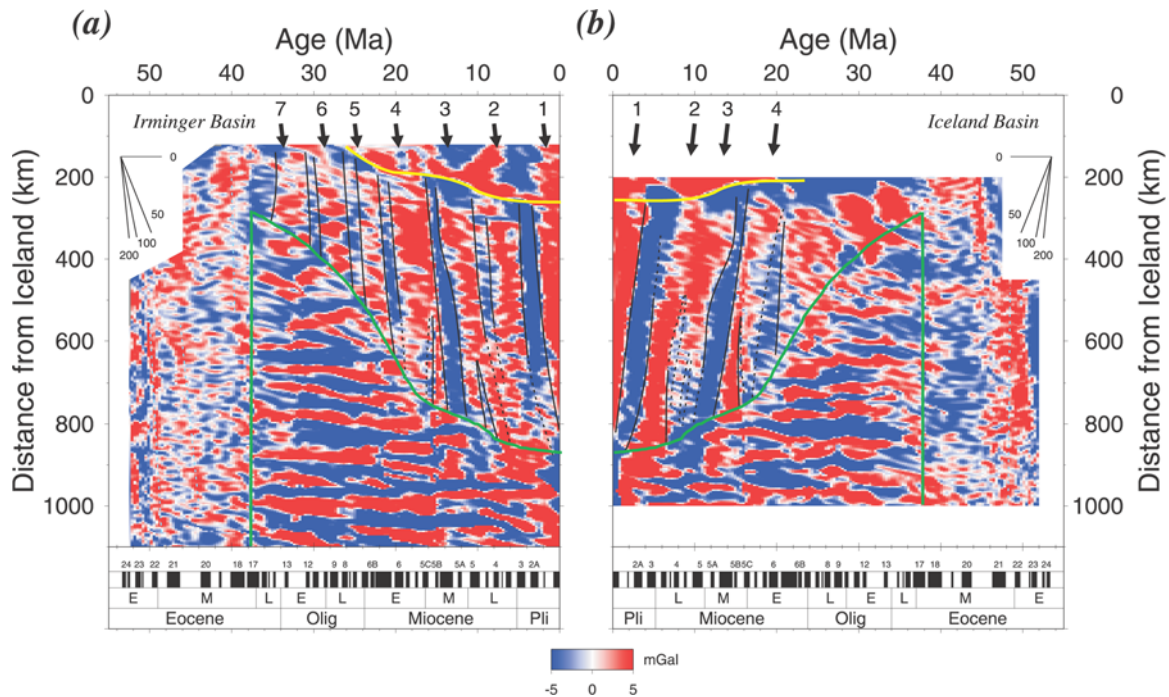
Figure 8. As Figure 7a and b, with interpretation superimposed. Black = V-shaped ridges. Green = boundary between segmented and unsegmented crust. Yellow = edge of Iceland Shelf. Light blue = indistinct gravity lineations of uncertain origin.
