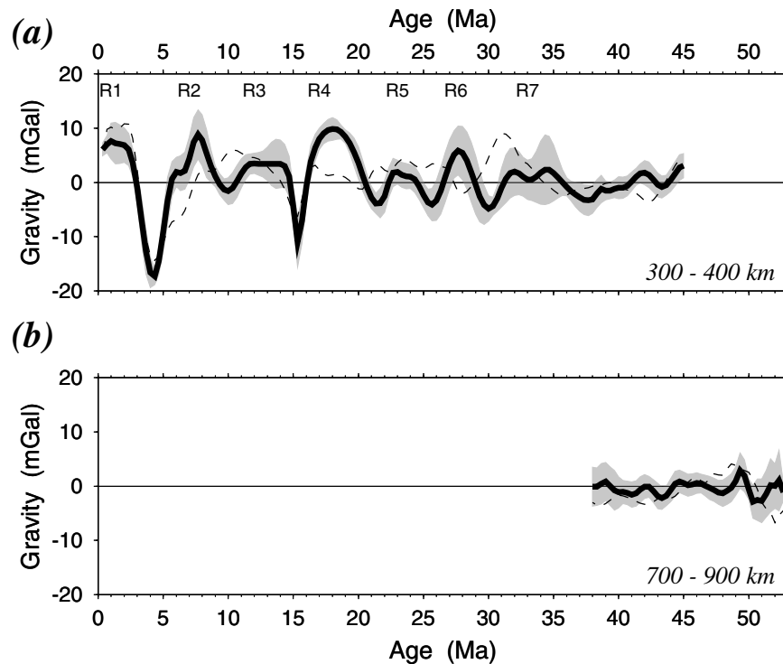
Figure 10. (a) Heavy black line marks the mean gravity profile across the Irminger Basin between 300–400 km from Iceland. Grey envelope marks the region of \pm 1 standard deviation. Thin black line is the mean profile across the Iceland Basin at the same distance. (b) Same for a distance of 700–900 km from Iceland.
