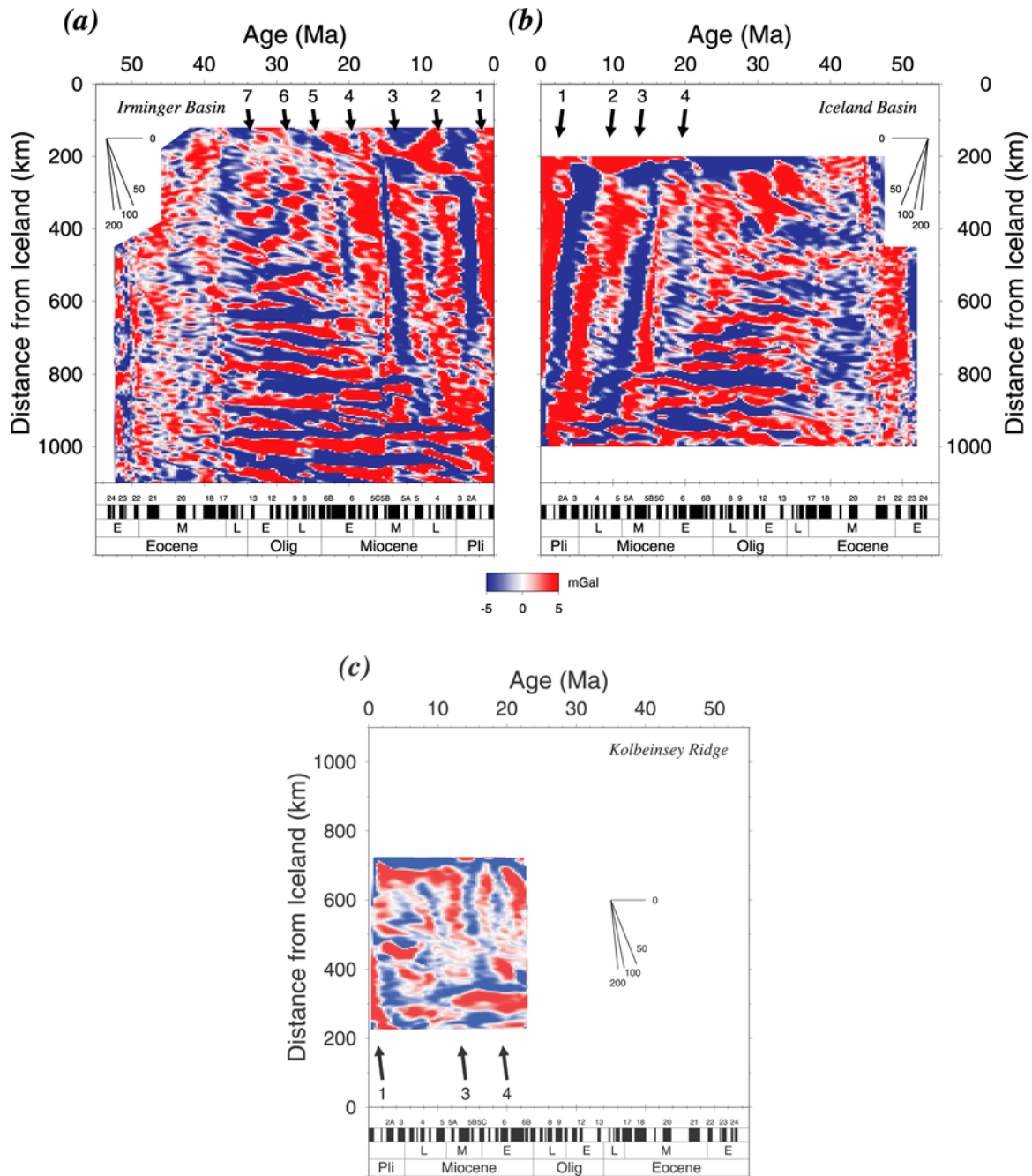
Figure 7. Age-distance plots of the short wavelength component of the gravity field over (a) the Irminger Basin, (b) the Iceland basin, and (c) the basin between the Kolbeisney Ridge and the Jan Mayen continental fragment. Numbered arrows above each plot refer to the scheme used to describe V-shaped ridges in the text and other figures. Numbered lines below name of each basin indicate propagation speeds in \text{km Myr}^{-1} for features lying at various angles. Black bars below each plot mark normally magnetised chrons from the geomagnetic timescale of Cande and Kent [1995] and adjacent numbers mark the chrons identified around Iceland in this study.
