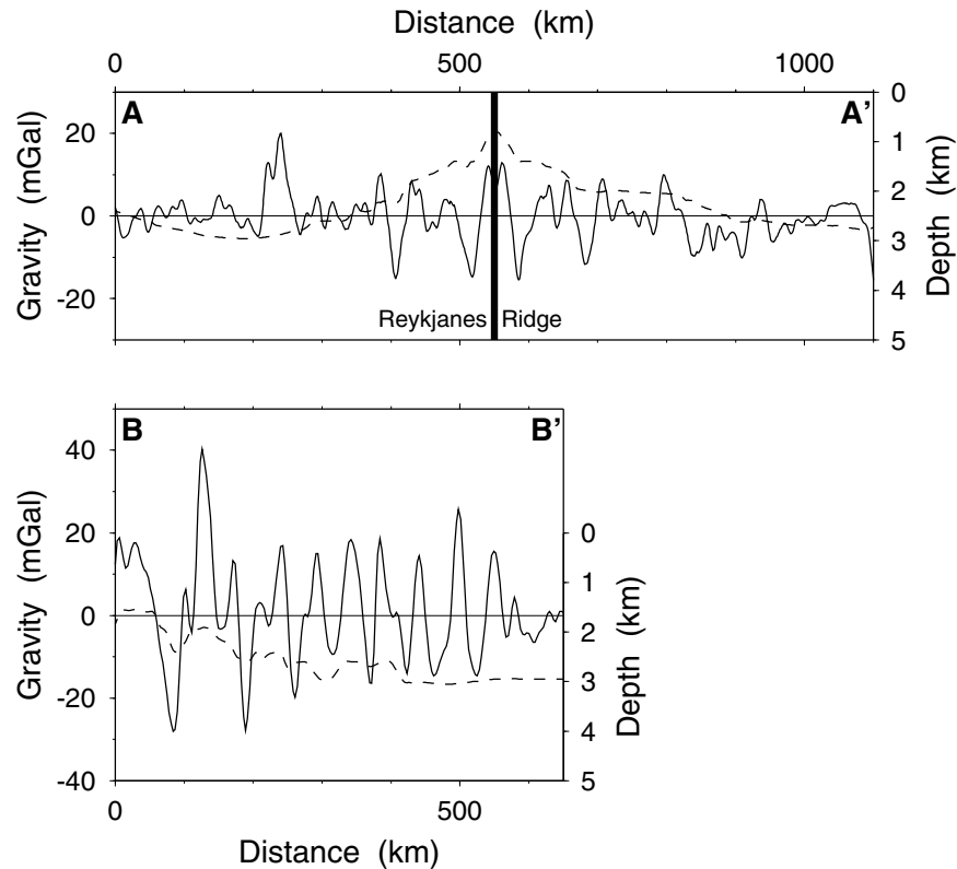
Figure 11. Free-air gravity profiles (solid lines) to illustrate the wavelength and amplitude of the anomalies associated with V-shaped ridges and fracture zones. Topographic profiles from ETOPO5 are shown as dashed lines. Vertical line marks spreading centre. Locations of profiles marked on Figure 4.
