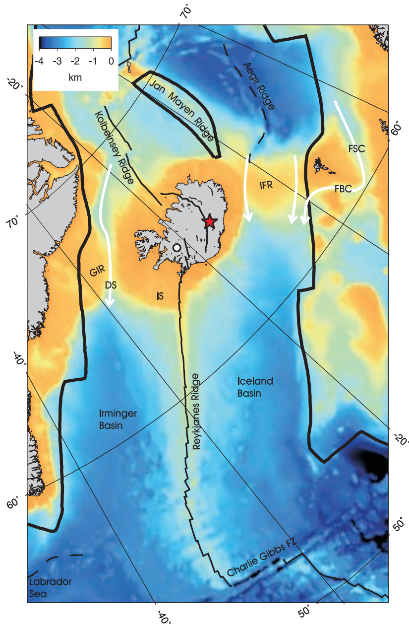
Figure 1. Location map showing physical features discussed in the text superimposed on the ETOPO5 topography field. Heavy black lines mark continent–ocean boundaries. Red star marks the present day center of the Iceland Plume; white circle marks the origin for distance measurements in Figures 7–9. White arrows show pathways for influx of Northern Component Water, generated north of Iceland, into the global ocean system. DS = Denmark Strait; FBC = Faroe Bank Channel; FSC = Faroe Shetland Channel; GIR = Greenland-Iceland Ridge; IFR = Iceland-Faroes Ridge.
