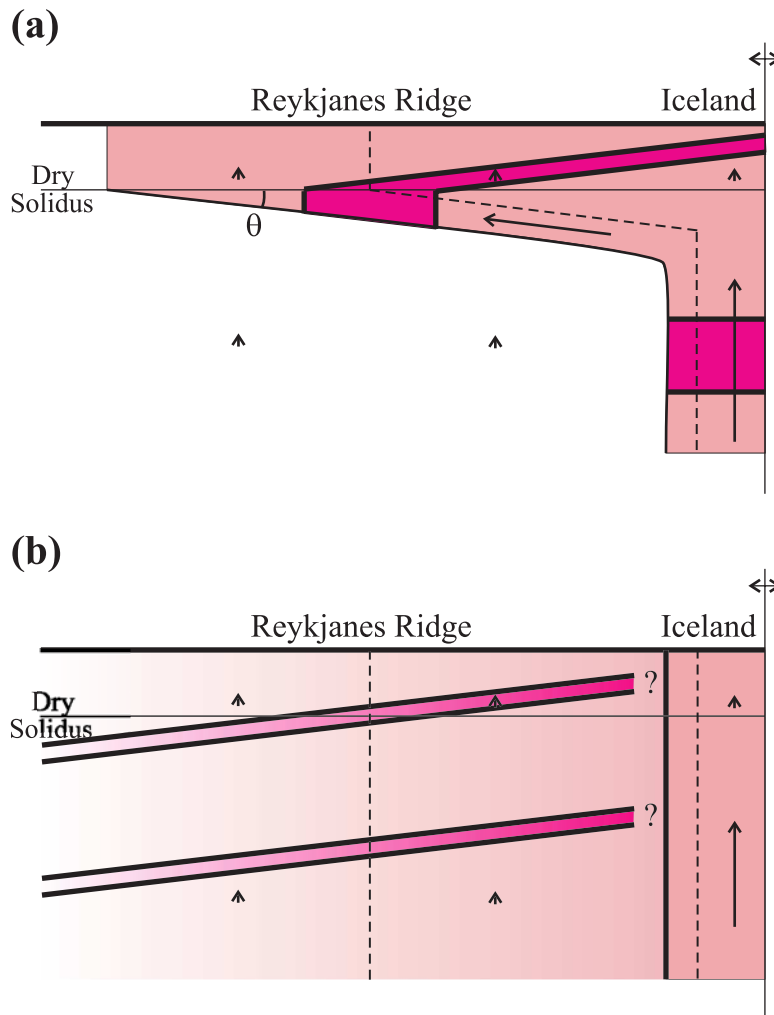
Figure 3. Schematic vertical sections through the upper mantle in the plane of the spreading axis, showing two geometries of temperature anomalies that could kinematically explain the V-shaped ridges. Dashed lines are flow stream lines and arrow lengths give an indication of relative flow speeds. Colors provide an indication of temperature; white represents normal temperatures and pinker shades represent anomalously high temperatures. Model (a) is characterised by both horizontal and vertical flow. Mantle viscosity increases significantly above the dry solidus occurs as dehydration occurs [Ito et al. , 1999]. Below the dry solidus a combination of horizontal flow in the plume head and vertical flow in response to plate separation occurs. Above the dry solidus only vertical flow occurs. Model (b) is characterised by vertical-only flow at all depths. See section 2 for further explanation.
