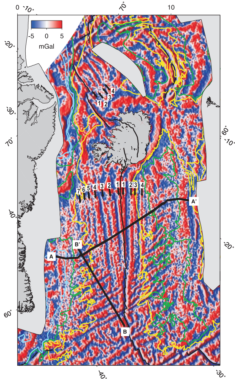
Figure 4. Short-wavelength component of satellite gravity field, related to variations in the thickness and structure of oceanic crust. The long-wavelength gravity field was calculated using a Gaussian filter of radius 100 km and subtracted from the original field to give the short-wavelength field. Numbered arrows refer to the scheme used to describe V-shaped ridges in the text and other figures. Coloured lines indicate sediment thickness after Srivastava et al. [1988]; yellow = 500 m; green = 1 km; blue = 1.5 km, 2 km and 2.5 km. Lines A–A' and B–B' mark locations of profiles in Figure 11.
