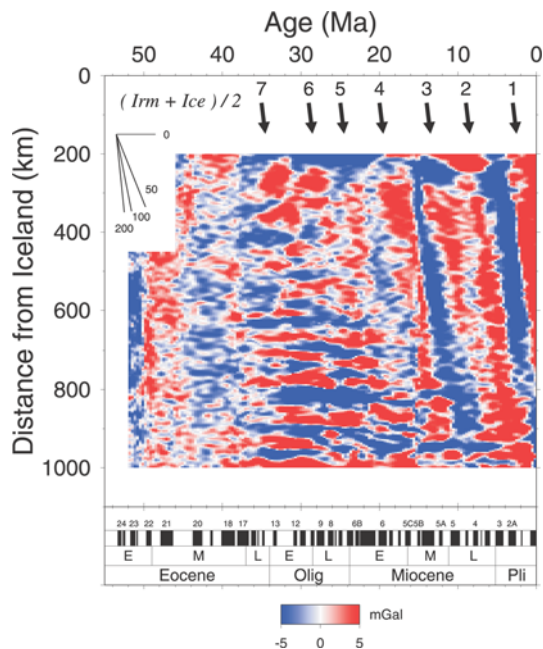
Figure 9. (a) Stacked age-distance plot for gravity record of V-shaped ridges in the Irminger and Iceland Basins. Stratigraphic data as for Figure 7.
