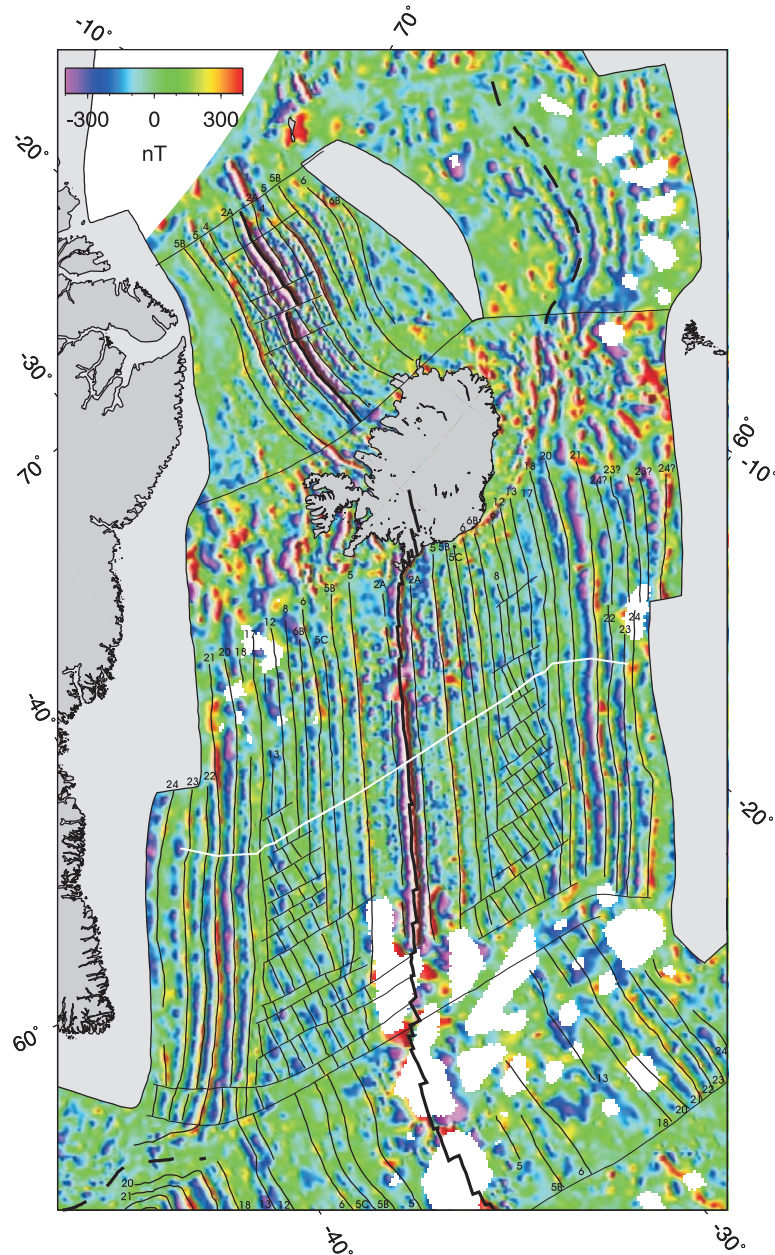
Figure 5. Magnetic anomaly compilation of Macnab et al. [1995]. White regions contain no data. Black lines mark magnetic anomalies picked and used in this study. White line marks plate-spreading flowline calculated from the poles of Smallwood and White [2002].
