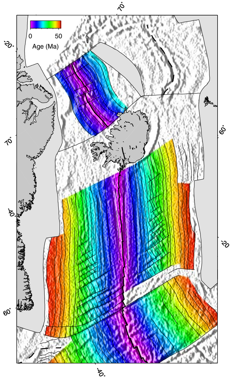
Figure 6. Age map from gridding the magnetic anomaly data picked from Figure 5. Gridding was done with continuous curvature splines [Smith and Wessel, 1990], and picks within each fracture zone-bounded segment were gridded separately and then combined to produce sharp discontinuities at the fracture zones. Grey-scale shading indicates the relief of the short-wavelength gravity field (Figure 4). Note good correlation between fracture zones picked from the magnetic dataset and the gravitational signature of fracture zones.
