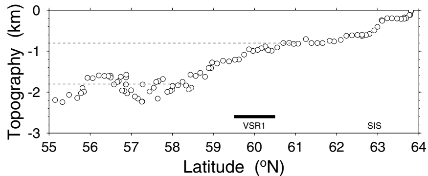
Figure 15. Bathymetric profile along Reykjanes Ridge taken from ETOPO5. Dashed lines indicate the step in bathymetry where V-shaped ridge R1 intersects the Reykjanes Ridge. VSR1 = intersection of V-shaped ridge R1 and Reykjanes Ridge; SIS = southern edge of Iceland Shelf.
