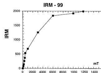
Figure 9. Results of rock-magnetic and demagnetization experiments for the Badin formation of Mogzon region (Late Jurassic). (a) and (b) Typical orthogonal vector plots (Zijderveld 1967), in tilt-corrected coordinates, for thermal (steps indicated in °C) and AF (steps indicated in mT) demagnetizations. Symbols: same conventions as in Fig. 3. (c) IRM acquisition in fields of up to 1.2 T showing the presence of both low-coercivity (left, sample 43) and high-coercivity (right, sample 99) magnetic minerals.
