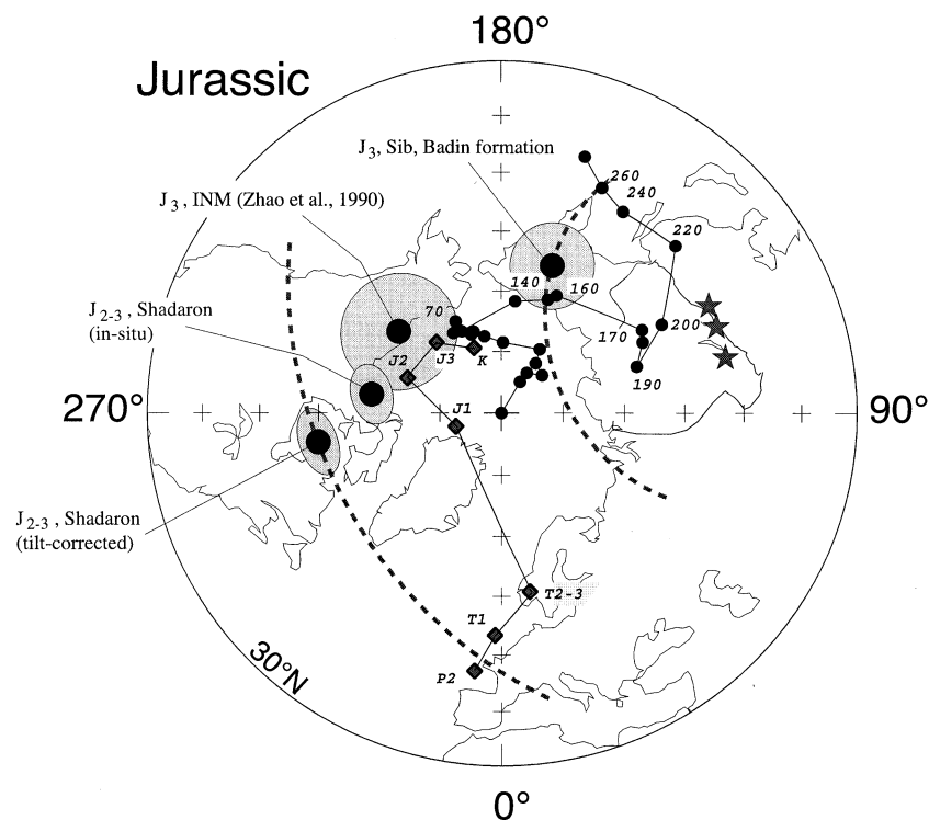
Figure 12. Equal-area projection of the northern hemisphere of the Early, Middle and Late Jurassic palaeopoles (large dots with dp/dm ellipses of confidence) from the present study. Small dots, diamonds, stars and dotted curves are as in Fig. 11. INM: Inner Mongolia block. Sib: Siberia.
