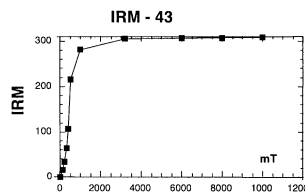
Figure 9. Results of rock-magnetic and demagnetization experiments for the Badin formation of Mogzon region (Late Jurassic). (a) and (b) Typical orthogonal vector plots (Zijderveld 1967), in tilt-corrected coordinates, for thermal (steps indicated in °C) and AF (steps indicated in mT) demagnetizations. Symbols: same conventions as in Fig. 3. (c) IRM acquisition in fields of up to 1.2 T showing the presence of both low-coercivity (left, sample 43) and high-coercivity (right, sample 99) magnetic minerals.
