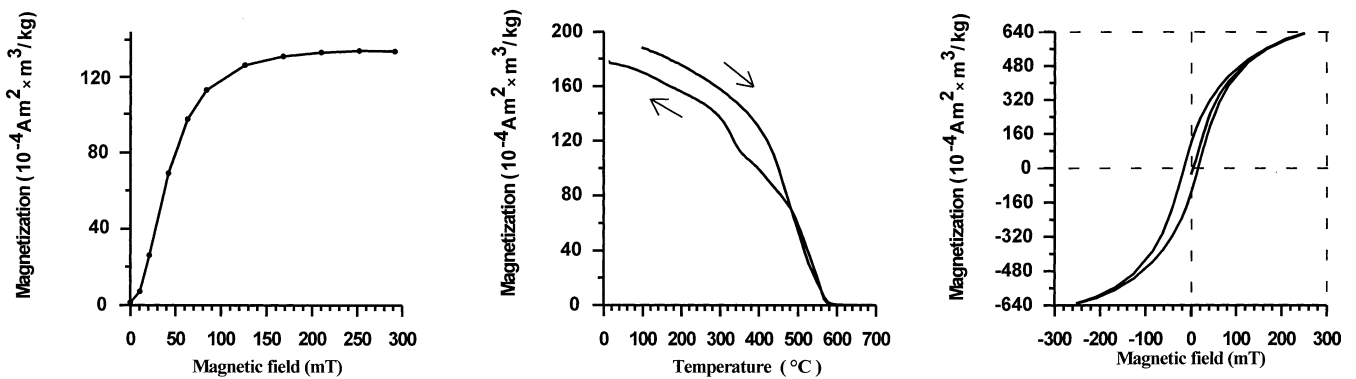
Figure 11. Results of rock magnetic experiments for Late Devonian–Early Carboniferous traps of the Markha and Viluy rivers. IRM acquisition curves (left), Curie point thermomagnetic curves J_s(T) (centre) and hysteresis loops (right).
