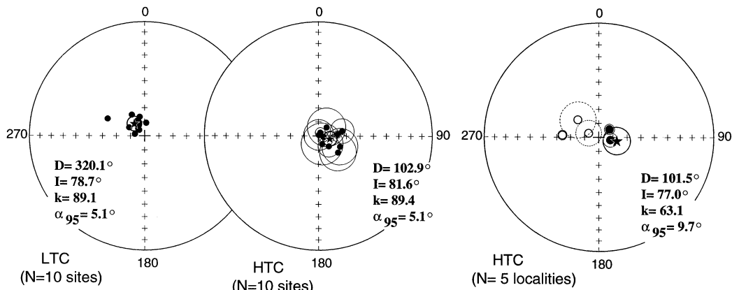
Figure 17. (a) Results of thermal and AF demagnetization of Late Permian–Early Triassic trap sill samples from the Aikhal kimberlite pipe area. See Fig. 4 legend for further details. Equal-area projections of site-mean directions of LTC and HTC, with circles 95 per cent of confidence shown in in situ coordinates. (b) LTC and HTC for the Late Permian–Early Triassic trap sill of the Aikhal kimberlite pipe area. (c) HTC for all Late Permian–Early Triassic trap sills (area of Sytikanskaya, Yubileynaya and Aikhal kimberlite pipes) and overprint directions of Mir and Sputnik kimberlite pipes. Other details as in Fig. 4.
