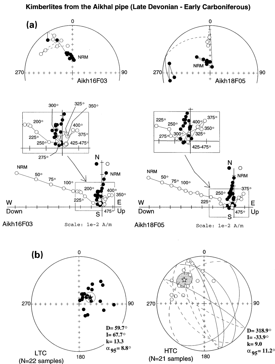
Figure 6. (a) Results of thermal demagnetization of Aikhal kimberlite pipe and satellite body samples. (b) Equal-area projections of site-mean directions of LTC and HTC, with circles of 95 per cent confidence for the Aikhal kimberlite pipe (Late Devonian–Early Carboniferous). See Fig. 4 legend for further details.
