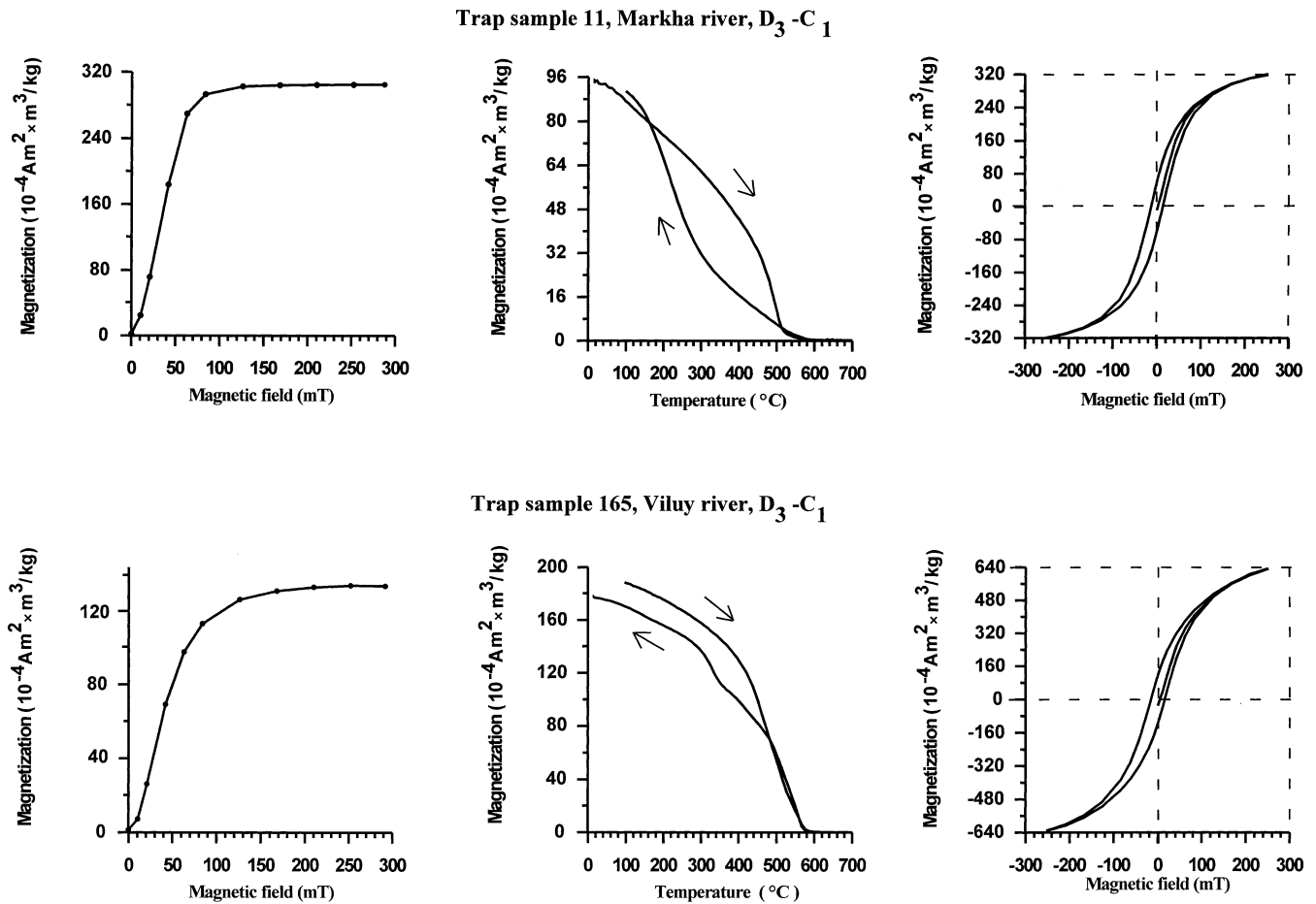
Figure 11. Results of rock magnetic experiments for Late Devonian–Early Carboniferous traps of the Markha and Viluy rivers. IRM acquisition curves (left), Curie point thermomagnetic curves J_s(T) (centre) and hysteresis loops (right).
