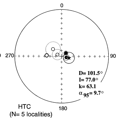
Figure 17. (a) Results of thermal and AF demagnetization of Late Permian–Early Triassic trap sill samples from the Aikhal kimberlite pipe area. See Fig. 4 legend for further details. Equal-area projections of site-mean directions of LTC and HTC, with circles 95 per cent of confidence shown in in situ coordinates. (b) LTC and HTC for the Late Permian–Early Triassic trap sill of the Aikhal kimberlite pipe area. (c) HTC for all Late Permian–Early Triassic trap sills (area of Sytikanskaya, Yubileynaya and Aikhal kimberlite pipes) and overprint directions of Mir and Sputnik kimberlite pipes. Other details as in Fig. 4.
