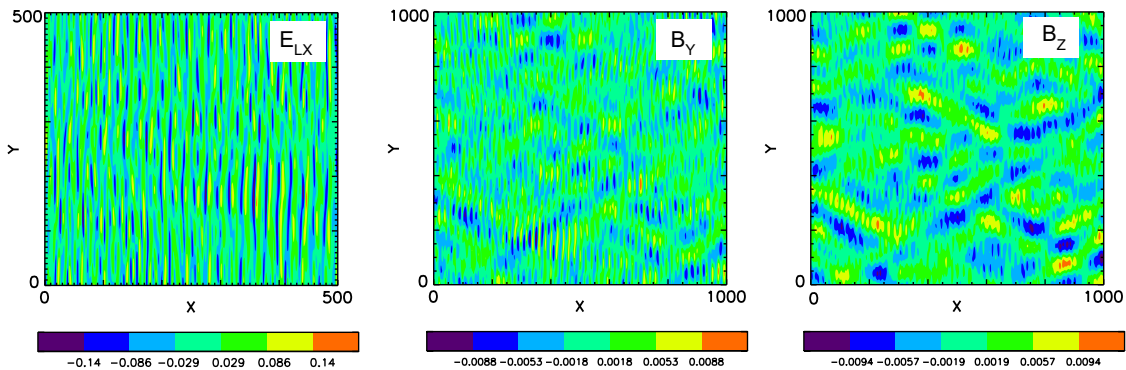
Figure 1. Snapshot of some field components shown on a portion of the simulation grid ( \mathbf{B}_0 parallel to y ).
