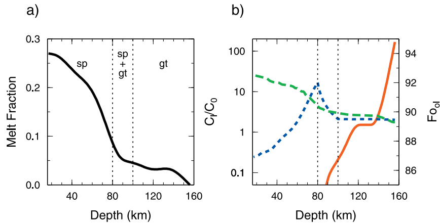
Figure 11. (a) Best fitting melt fraction against depth model for Theistareykir [Maclennan et al. , 2003]. The dashed lines mark the depths of the spinel-garnet transition. (b) Predicted instantaneous fractional melt compositions from the model in Figure 11a. The La and Yb concentrations are shown normalized to the mantle source composition (left axis). La is shown as a solid red line and Yb as a short-dashed blue line. The green long-dashed line shows the calculated forsterite content of the olivine in equilibrium with the fractional melts.
