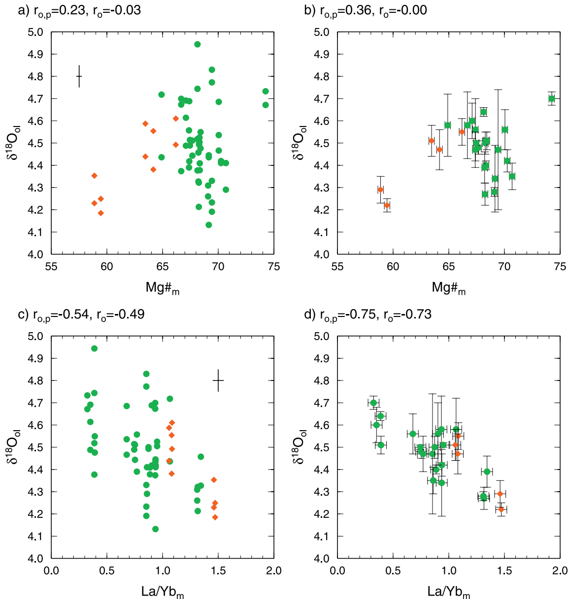
Figure 14. Oxygen isotope data from Eiler et al. [2000]. Figures 14a and 14c show the \delta^{18}\text{O} of individual crystals plotted against their host sample composition, while Figures 14b and 14d show the average \delta^{18}\text{O} of crystals in a sample plotted against the sample composition. The green circles show \delta^{18}\text{O}_{ol} measurements that were made on olivine crystals. The red diamonds show \delta^{18}\text{O}_{ol} predicted from \delta^{18}\text{O} on plagioclase using the high-temperature fractionation of \sim 0.6 per. mil. from Chiba et al. [1989]. The error bars in Figures 14a and 14c show the 1\sigma precision error for each point, while those for \delta^{18}\text{O}_{ol} in Figures 14b and 14d are the 1\sigma variability of the measurements in each sample. The \text{Mg}\# of the melt was taken from the calculation of Eiler et al. [2000], who corrected the composition of each sample for the effect of olivine accumulation. The correlation coefficients are shown both for the entire data-set, r_{o,p} , and for the measurements made on olivine crystals alone, r_o .
