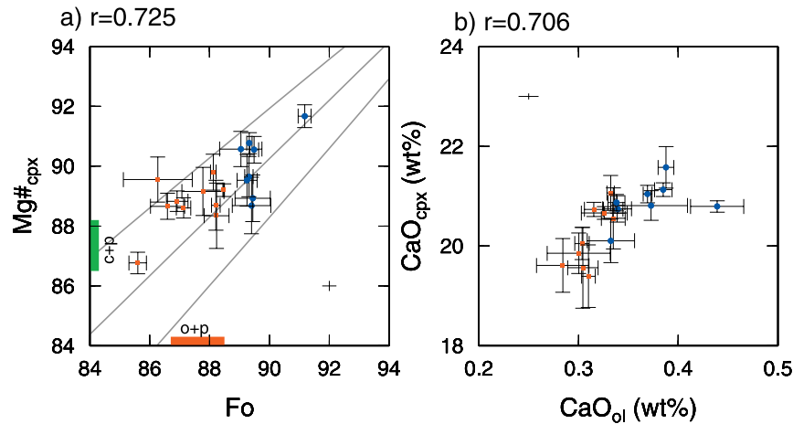
Figure 7. Average clinopyroxene compositions plotted against average olivine compositions from nodules where clinopyroxene and olivine are both present. The error bars show 1\sigma variation within individual nodules. Red squares show nodules where plagioclase is present, blue circles show those where only clinopyroxene and olivine are present. The cross without a point shows the 1\sigma analytical precision. The red bar marked o + p in Figure 7a shows the range of olivine compositions found in the troctolites, while the green bar marked c + p shows the range of clinopyroxene compositions in olivine-free gabbros. The grey lines in Figure 7a show the equilibrium Fe-Mg partitioning calculated using the method of Loucks [1996], for temperatures of 1160°C (upper line), 1210°C and 1260°C.
