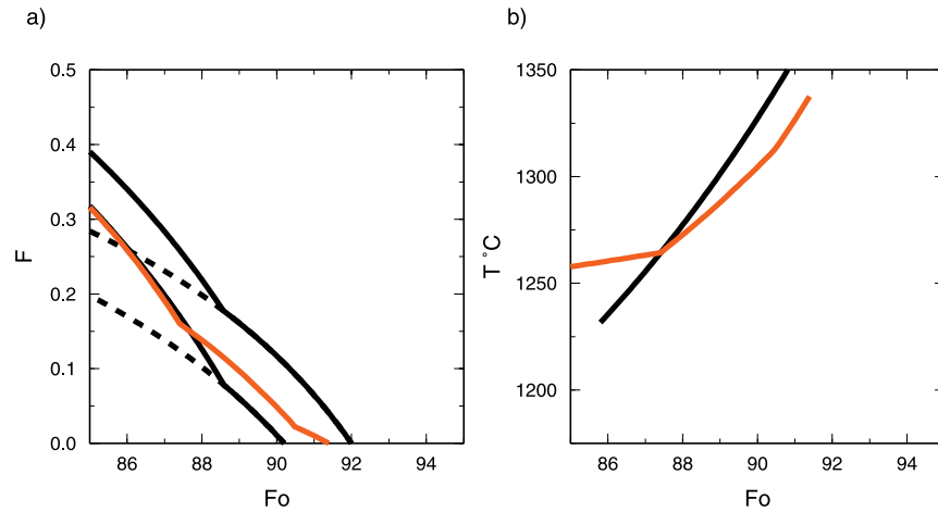
Figure 12. (a) Black lines show the relationship between fraction crystallized, F , and the forsterite content of the equilibrium olivine for two different starting compositions. The dashed black lines show the predicted F for crystallization of phases with K_d \sim 0.3 only (olivine, clinopyroxene) and were calculated using Equation 6. The solid line shows the predicted F if 50% of the crystallizing assemblage consists of plagioclase at forsterite contents of less than 88.6 mol%. The red line shows the relationship between F and F_o obtained using the model of Weaver and Langmuir [1990] with the average Borgarhraun melt as a starting composition [MacLennan et al. , 2003], a pressure of 0.8 GPa and an oxygen fugacity held at one log unit beneath the quartz-fayalite-magnetite buffer. (b) The black solid line is the relationship between temperature and F_o for Borgarhraun samples calculated using the thermometer of Roeder and Emslie [1970] as described in the text. The red line shows the relationship for the Weaver and Langmuir [1990] fractionation model detailed in Figure 12a.
