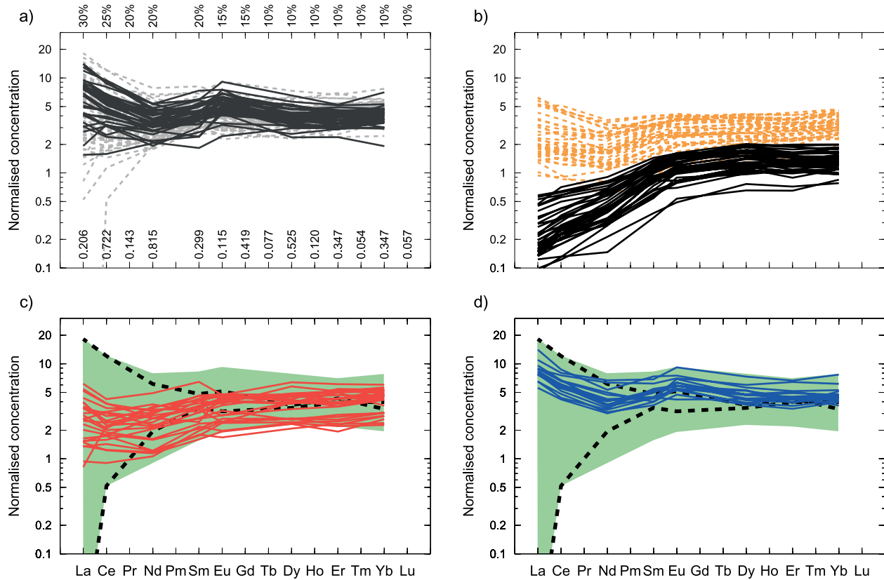
Figure 2. Depleted mantle source normalized REE measurements (a) Olivine hosted melt inclusion compositions from Borgarhraun nodules are shown as black lines. Borgarhraun phenocryst olivine-hosted melt inclusions from Slater et al. [2001] and Maclellan et al. [2003] are shown as grey dashed lines. The values at the bottom of the plot show the composition of the depleted mantle source of McKenzie and O’Nions [1991] that is used for normalization and those at the top show the estimated mantle error on this source composition. (b) Borgarhraun nodule clinopyroxene compositions are shown as black lines. The orange lines show the range of melt compositions in equilibrium with the clinopyroxenes, calculated using the method of Wood and Blundy [1997] as described in section 4.2 of the text. (c) Green field shows that total range of composition of melt inclusions hosted in olivines with forsterite contents <90.6. The red lines show the compositions of melt inclusions hosted in olivines with >90.6. The upper black dashed line shows the composition of the melt inclusion with the highest La/Yb, and the lower one shows the composition of the melt inclusion with the lowest La/Yb. (d) Same as Figure 2c, except that the blue solid lines show the composition of melt inclusions hosted in olivines with forsterite contents of <87.5.
