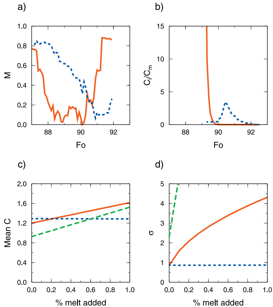
Figure 13. (a) Comparison of observed M for La (solid red line) and Yb (dotted blue line). (b) Predicted composition of instantaneous fractional melts from Theistareykir melting model (See Figure 11). The instantaneous compositions, C_i are shown here normalized to the mean predicted melt composition, C_m , from the melting model. The solid red line is La and the dotted blue one is Yb. (c) Variation in average composition caused by addition of extreme initial melts from the melting model to the distribution of melt inclusion compositions found at Fo_{90} . This variation was calculated using equation (9). The La concentration (ppm) is shown in a solid red line, the Yb concentration (ppm) in a dotted blue line and the La/Yb ratio in a green dashed line. (d) Variation in standard deviation of the sample caused by introduction of extreme initial melts to the distribution of melt inclusion compositions found at Fo_{90} . This variation was calculated using equation (10). The lines have the same colors as those used in Figure 13c.
