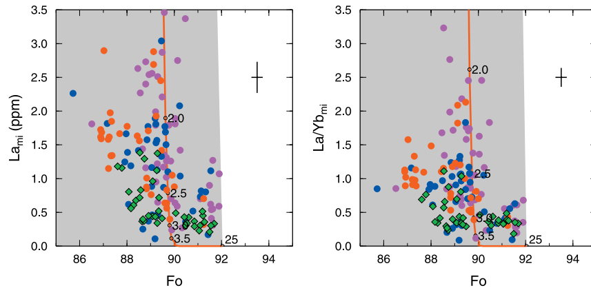
Figure 8. REE compositions of Borgarhraun melt inclusions plotted against forsterite content of their host olivines. The blue circles show the phenocryst data of Maclennan et al. [2003], the purple circles the phenocryst data of Slater et al. [2001] and the red circles the nodule data from this work. The green diamonds show the nodule clinopyroxene compositions converted into melt and equilibrium olivine composition as described in the text. The red line shows the path of instantaneous fractional melt compositions from the melting model in Figure 11. The line is labeled with the percent of melting required to generate the melt compositions. The first melts are in equilibrium with a FO_{89} olivine and have a La content of 43 ppm and a La/Yb ratio of 61 and are too extreme to be displayed on these plots. The grey region shows the field of all possible melt/olivine compositional pairs that can be generated by mixing and fractional crystallization of the predicted instantaneous fractional melt compositions. The black cross shows the 1\sigma analytical precision calculated from repeat measurements.
