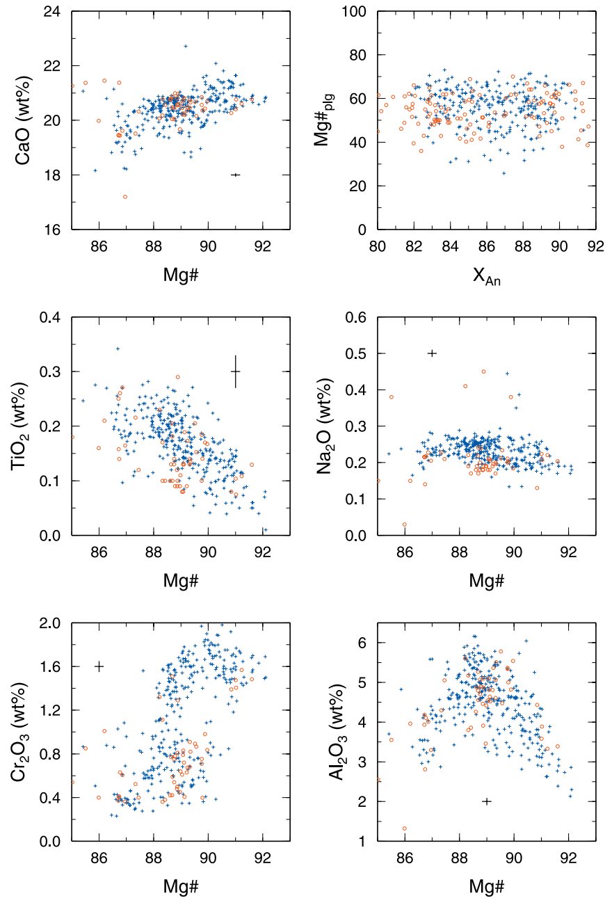
Figure 5. Comparison of mineral phases from nodules and phenocrysts, using same symbols as Figure 4. The plots are all for clinopyroxene compositions save the upper right which shows plagioclase compositions.
