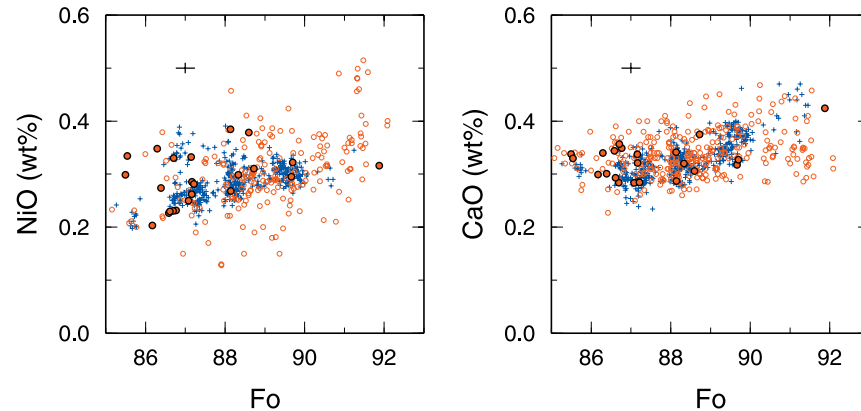
Figure 4. Comparison of olivine compositions from nodules (small blue crosses) and phenocrysts (unfilled red circles). Measurements from skeletal olivine phenocrysts are shown as filled red circles with a thick black outline. The \pm 1\sigma analytical precision is shown as a black cross.
