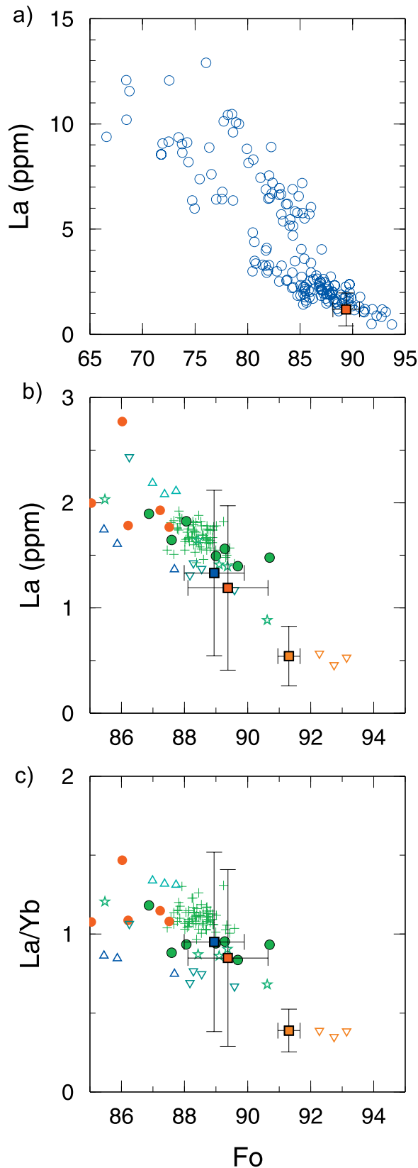
Figure 6. (opposite) (a) Plot of all Theistareykir glacial and postglacial compositions reported by MacleNNan et al. [2002] from Slater [1996] are shown as blue circles. The La concentration is that of the whole rock sample and the Fo content is that calculated to be in equilibrium with the whole rock composition at a temperature of 1200°C and a pressure of 0.8 GPa using the method of Ford et al. [1983]. The calculated K_d^{Fe-Mg} was 0.32 \pm 0.01 . The Fe^{3+} to Fe^{2+} ratio of the melt was calculated at an oxygen fugacity one log unit beneath the quartz-fayalite-magnetite buffer using the method of Kilinc et al. [1983]. This method gave an average Fe^{2+}/Fe^{tot} of 0.90 \pm 0.01 . The red filled square shows the mean composition of the Borgarhraun melt inclusions and their host olivines with the error bars showing 1\sigma . (b) Detailed comparison between average Borgarhraun melt inclusion compositions and Theistareykir whole-rock compositions. The whole rock data in this plot are the high precision measurements of Stracke et al. [2003] of primitive Theistareykir samples and the Borgarhraun analyses of MacleNNan et al. [2003]. The red filled square is the mean melt inclusion and host olivine composition, the blue filled square is the mean in host olivines with Fo < 90.6, and the brown filled square is the mean in host olivines with Fo > 90.6. The whole rock symbols are as follows. Brown downward pointing triangles, picrites; dark green downward pointing triangles, Hoefudreidarmuli; blue upward pointing triangles, Arnahvammurhraun; turquoise upward pointing triangles, Bondholshraun; small red filled circles, Storaviti; green stars, Langaviti; filled green circles, Borgarhraun [Stracke et al. , 2003]; green crosses, Borgarhraun [MacleNNan et al. , 2003]. (c) Same key as for Figure 6b.
