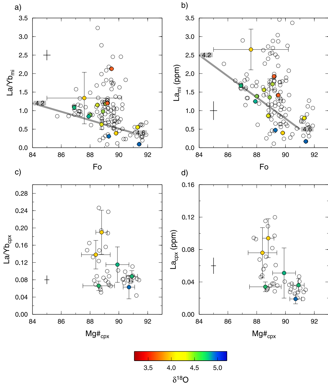
Figure 16. Relationship between REE and major element content and \delta^{18}\text{O} of olivines, clinopyroxenes and melt inclusions. Figures 16a and 16b show the same data as Figure 8, with the addition of a number of colored points showing the \delta^{18}\text{O} of the host olivine. The color scale for \delta^{18}\text{O} is given at the base of the figure. The error bars on the colored points show the variability within single crystals or nodules (for composite samples). The cross without a circle shows the 1\sigma analytical precision. The AFC trend proposed by Eiler et al. [2000] is shown as a thick grey line. This line is best fit to the Theistareykir whole-rock sample data from Eiler et al. [2000], with melt Mg#s converted into equilibrium olivine forsterite contents using a K_d^{\text{Fe-Mg}} of 0.3 and \text{Fe}^{2+}/\text{Fe}^{\text{tot}} of 0.9. The numbers on the grey boxes show the variation in \delta^{18}\text{O}_{\text{ol}} associated with this trend.
