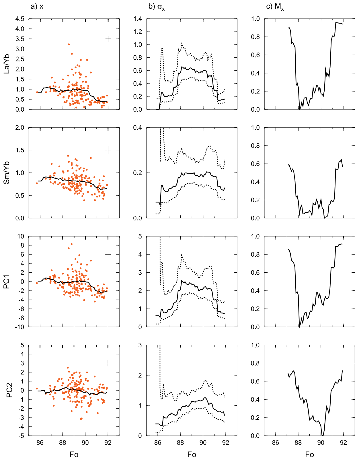
Figure 10. Same as Figure 9 but REE concentration ratios with respect to Yb are used instead of absolute concentrations. The principal components are given in Table 5.
