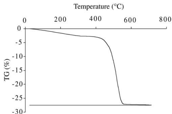
Figure 2. Thermal gravity analysis for samples heated from ambient temperature up to 700°C.
