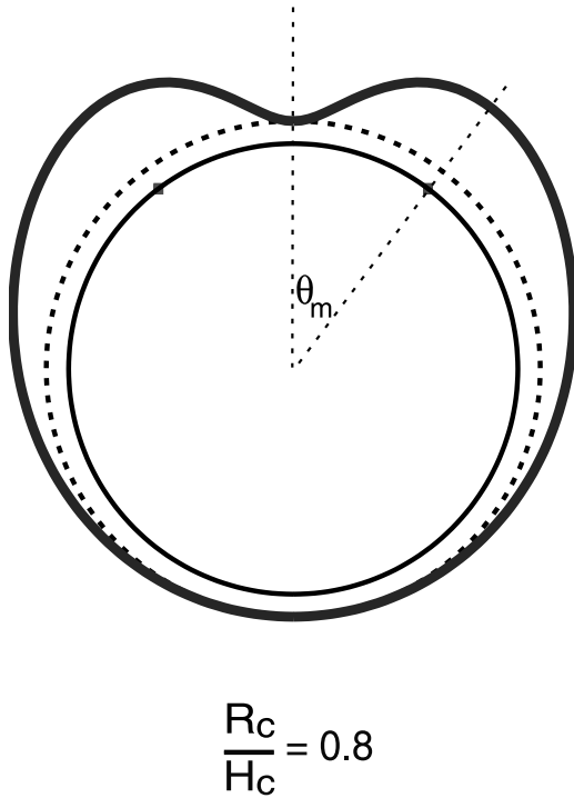
Figure 7. Angular distribution of hoop stress (thick plain curve) around the reservoir walls for the first elastic problem (magmatic overpressure and no edifice at the surface). Stress values are scaled by the magmatic overpressure \Delta P and are shown as a function of angle \theta for a_c = R_c/H_c = 0.8 (Figure 2). The top part of the diagram shows the convention used to draw the figure: compression and tension appear as negative and positive stresses, respectively (contrary to the sign convention used in the calculations). The thin plain circle corresponds to zero stress, and the dashed line shows a uniform tension of 1 corresponding to the solution in an infinite medium. The hoop stress is maximum for \theta = \theta_m such that \cos\theta_m = a_c .
