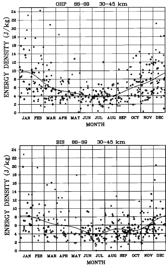
Fig. 2. Daily estimates of the potential energy density per unit mass in the upper stratosphere (30–45 km) observed during 4 years (86 to 89) and reduced into 1 year. A least squares fit by a linear combination of four sine and cosine functions (period of 12 to 3 months) is performed (smoothed curve).
