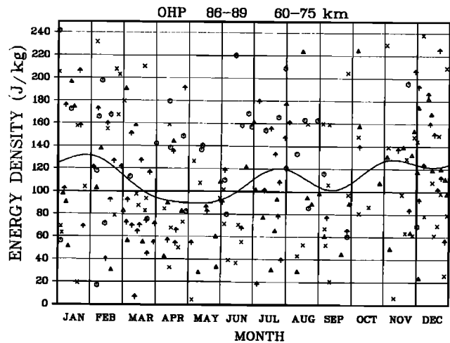
Fig. 7. The same as Figure 1 except in the middle mesosphere (60 to 75 km).
