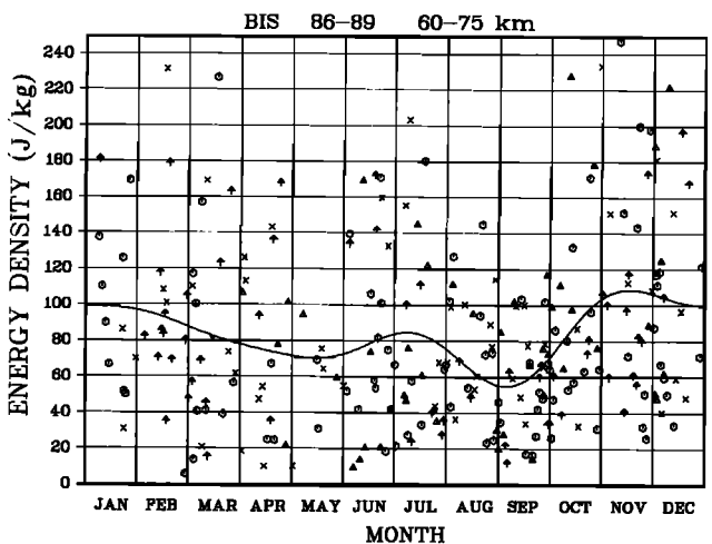
Fig. 8. The same as Figure 2 except in the middle mesosphere (60 to 75 km).
