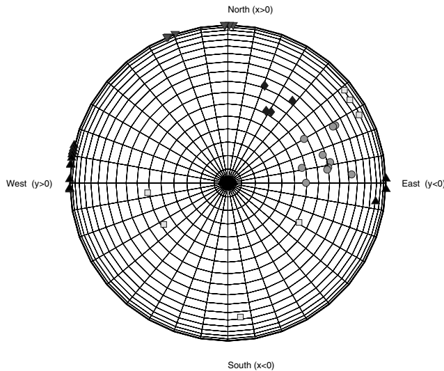
Figure 3. Orientation of the fracturation events in Table 1. Symbols correspond to the position of the vector \mathbf{n} on the unit sphere. Families 1, 2, 3 and 4 are denoted by \Delta , \circ , \diamond and \nabla , respectively. The line spacing is 10^\circ for the radial angle and 5^\circ for the inclination.
