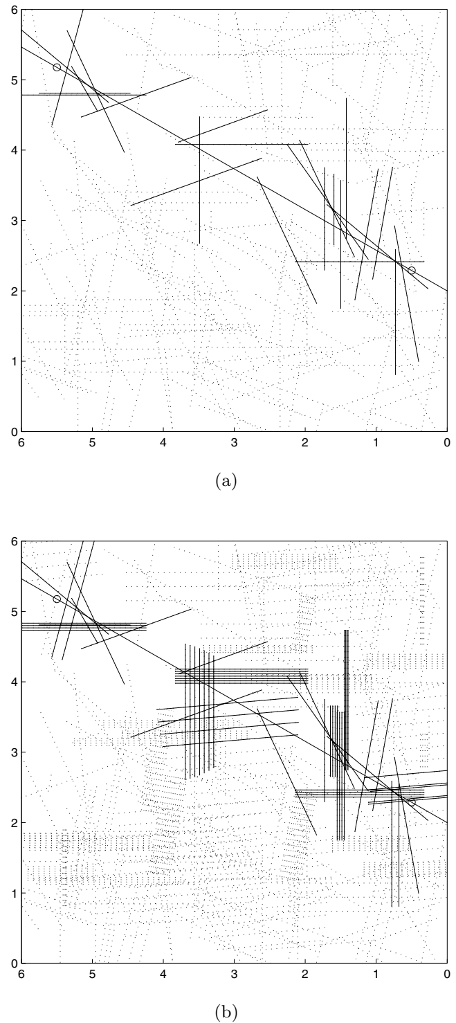
Figure 5. Trace maps obtained in an horizontal section through monodisperse reconstructed samples. The cell size is L = 600 m and the event radius R = 100 m. The events are represented by single fractures in (a) and as series of fractures in (b). The solid lines correspond to the traces of the events which intersect the 120^\circ N, 500 m long scan line (thick solid line). Traces in dotted lines do not intersect the scan line. Distances are in R units, i.e. 1:100 m.
