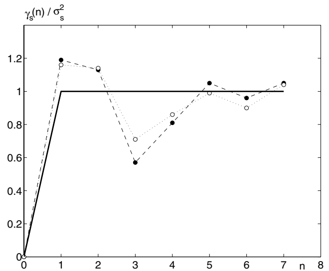
Figure 4. Variogram (30) of the spacings of the intersections of events from family F_1 with profile P_1 without (— \circ —) or with ( \cdots \circ \cdots ) inclusion of the part of the profile following the last observed intersection. The thick solid line corresponds to uncorrelated event locations.
