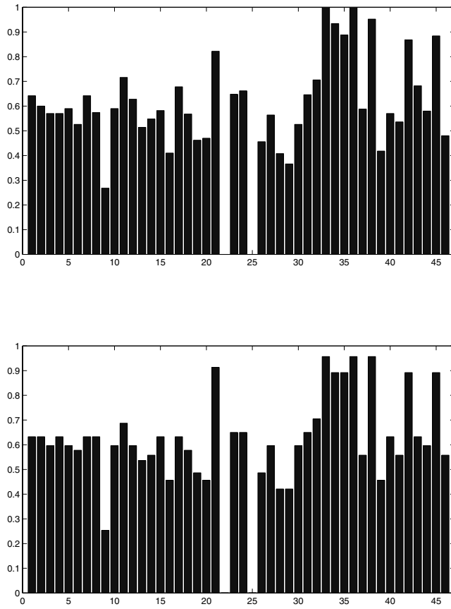
Figure 6. Mean number of event intersections with a 500 m long, 120°N scan line (see Fig. 5a). The abscissae correspond to the event number given in the first row of Table 1. Data in (a) correspond to the average over 500 monodisperse reconstructed samples, with L = 600 m, R = 50 m. Data in (b) are the expected values resulting from the field data.
