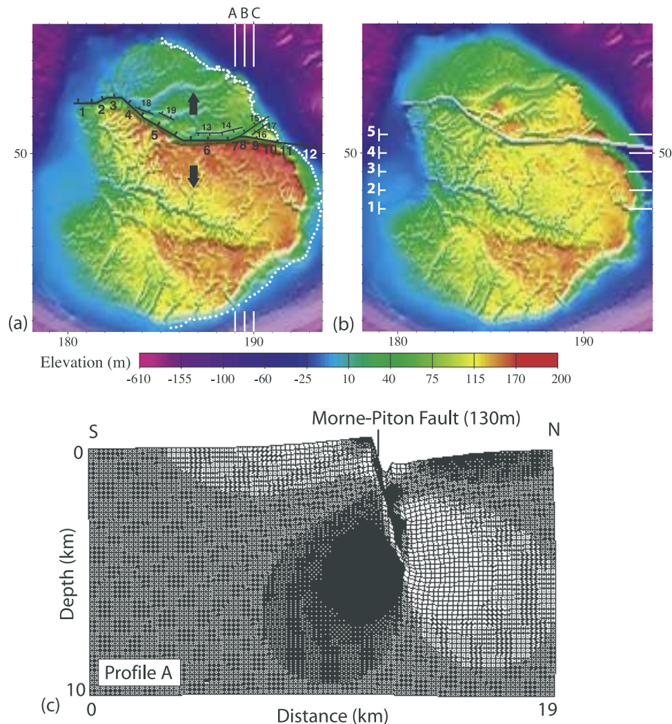
Figure 9. Morne-Piton fault modeling. Topography as in Figure 2b. Coordinates in km Mercator with the reference point at latitude 15^{\circ}30'N and longitude 63^{\circ}W . (a) Model in map view with present-day topography. Each fault segment is numbered (see Table 3). The Morne-Piton fault segments are modeled as dislocations (black lines with ticks, with thicker trace for higher slips) in an elastic half-space (see text). Double black arrows, direction of extension. The motion is dip slip on E-W striking faults. White lines with letters (A, B, C), location of topographic profiles shown on Figure 9c (profile A) and 10. White dots along coast, location of profile modeled in Figure 11 (see caption). (b) Residual topography, before motion of the Morne-Piton fault. Notice that the island remains clearly tilted westward. Numbered white lines, residual topographic profiles shown in Figure 13a. (c) Deformation model in section along the profile A (location Figure 9a). Vertical exaggeration 1. Each square is 200 m by 200 m. Dark shading, areas of dilatation; light shading, areas of compression. The main fault (Morne-Piton) is associated with a smaller antithetic fault. Both the footwall and the hanging wall of the main dislocation are flexed and tilted southward as observed for terraces (see text).
