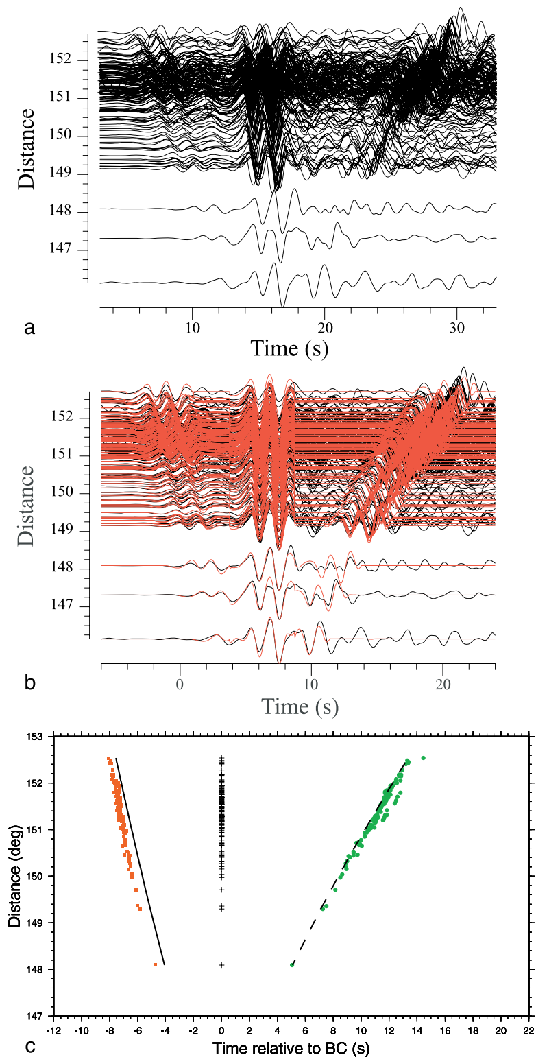
Figure 3. Example 1. (a) Raw data before inversion, aligned on the theoretical arrival time of PKP(BC) and plotted as a function of their epicentral distance (in degrees). (b) Data (black lines) and best model synthetic seismograms (red lines) aligned on the PKP(BC) phase. (c) Best model arrival times of the three PKP phases relative to PKP(BC) . Dashed lines indicate theoretical arrival times predicted by the ak135 reference Earth's model.
