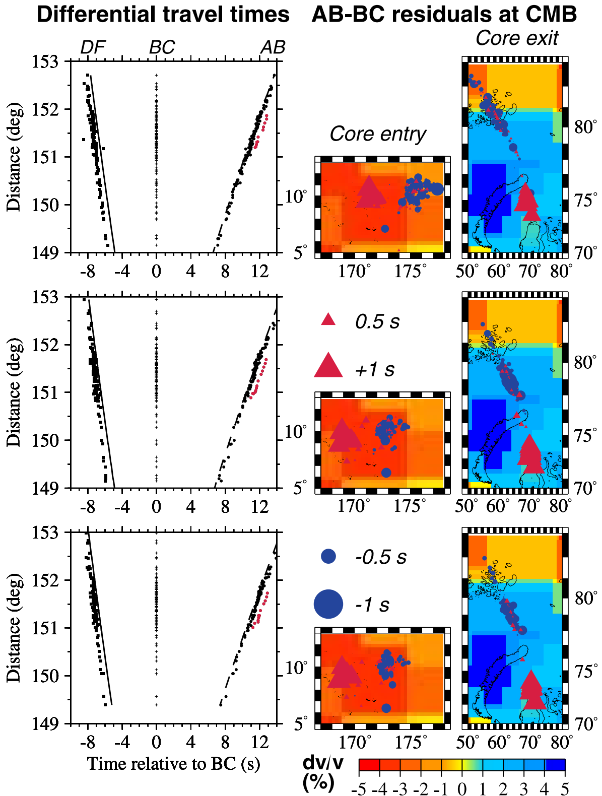
Figure 10. Interpretation of AB-BC differential travel time residuals. On the left, from top to bottom, differential travel times for events 2, 3, and 8 on Table 1. For each earthquake, the arrival times of the three core phases relative to PKP(BC) are plotted as a function of epicentral distance. The anomalous positive AB-BC residuals are shown in red, and the theoretical arrival times predicted by the ak135 Earth model are shown as solid and dashed lines. On the right, zero mean AB-BC differential travel time residuals are plotted at the entry and exit points in the core of the PKP(AB) rays, superimposed on the Bijwaard et al. [1998] P velocity model of the lowermost mantle. Positive AB-BC differential travel time residuals are shown with red triangles and negative residuals are shown with blue circles.
