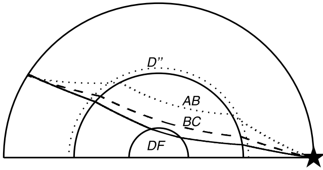
Figure 1. Ray paths of the three PKP branches in the Earth: PKP(DF) (solid line), PKP(BC) (dashed line) and PKP(AB) (dotted line). The event (black star) and the D'' layer at the base of the mantle are also indicated.
