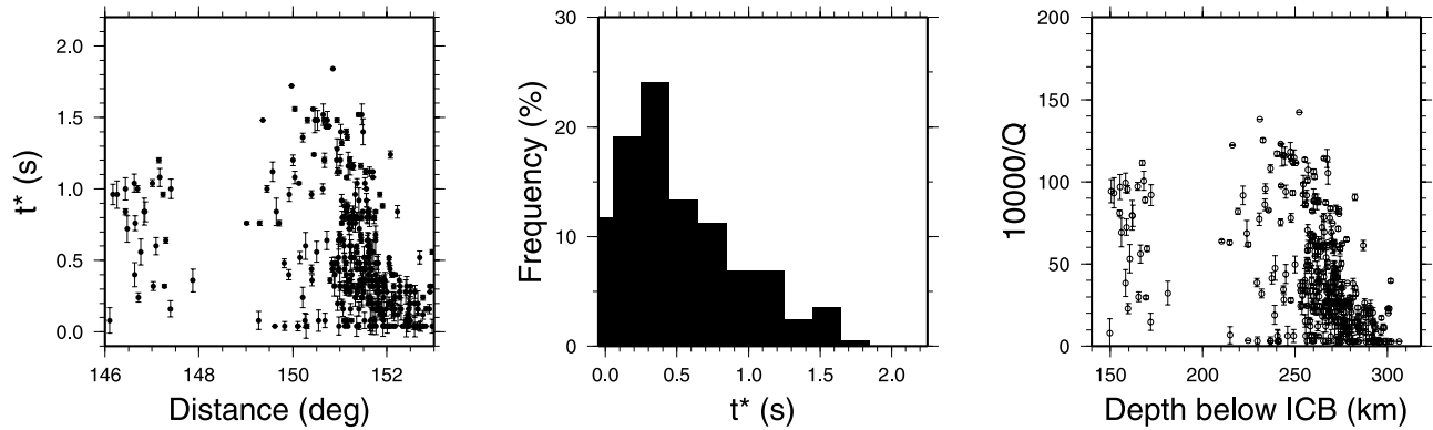
Figure 13. (left) BC-DF differential attenuation parameters t^* (s) as a function of epicentral distance ( ^{\circ} ). (middle) Histogram of BC-DF differential attenuation parameters t^* . (right) Inner core attenuation parameter q = 10,000/Q is shown as a function of depth of the PKP(DF) turning point in the inner core (km). Over the whole Eifel core phase data set, only t^* parameters presenting statistical errors lower than 0.1 s are plotted.
