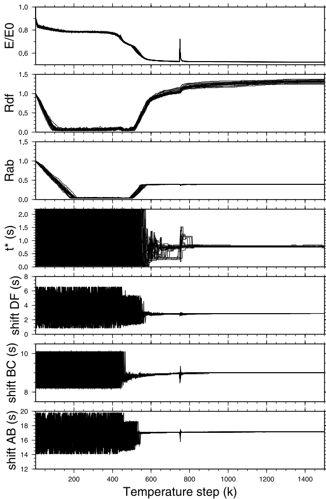
Figure 5. Energy, R_{DF} , R_{AB} and parameters of a randomly selected seismogram for the 20 SA inversions, as a function of the temperature step ( k ) describing the cooling schedule. From top to bottom: energy normalized to its starting value [ E(k)/E(0) ], R_{DF} , R_{AB} , parameter t_1^* in seconds, and parameters \tau_1^{DF} , \tau_1^{BC} , and \tau_1^{AB} in seconds.
