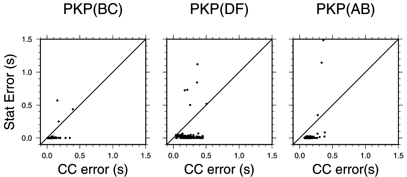
Figure 4. Statistical estimate of the time shifts RMS errors (in seconds) plotted as a function of the error computed for the best model using the cross correlation method described by Chevrot [2002]. From left to right, errors of the parameters \tau_i^{BC} , \tau_i^{DF} , and \tau_i^{AB} . The line indicates the one to one correspondence.
