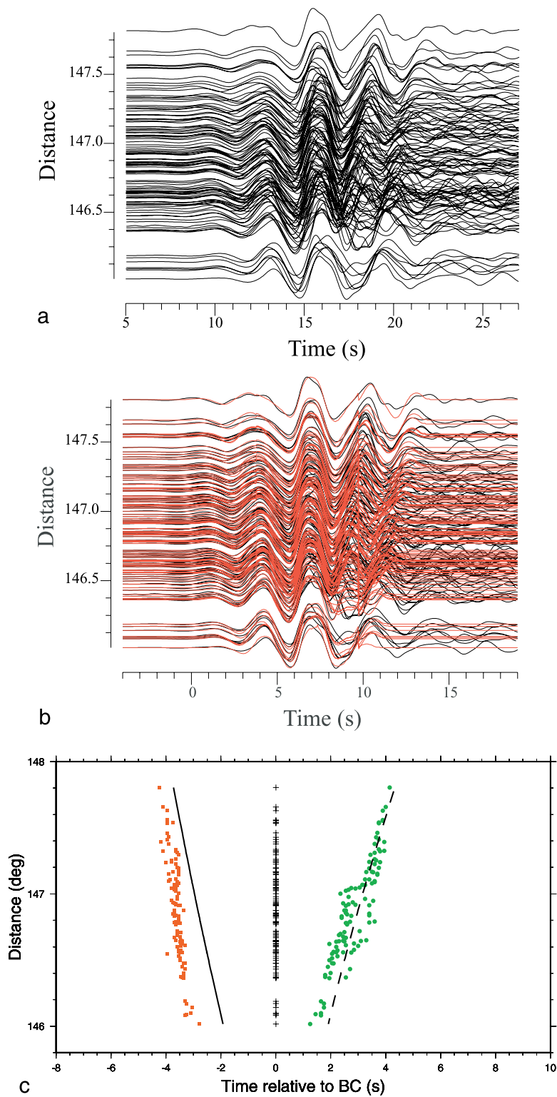
Figure 7. Example 2. (a) Raw data before inversion, aligned on the theoretical arrival time of PKP(BC) , and plotted as a function of their epicentral distance (in degrees). (b) Data (black lines) and best model synthetic seismograms (red lines) aligned on the PKP(BC) phase. (c) Best model arrival times of the three PKP phases relative to PKP(BC) . Dashed lines indicate theoretical arrival times predicted by the ak135 reference Earth's model.
