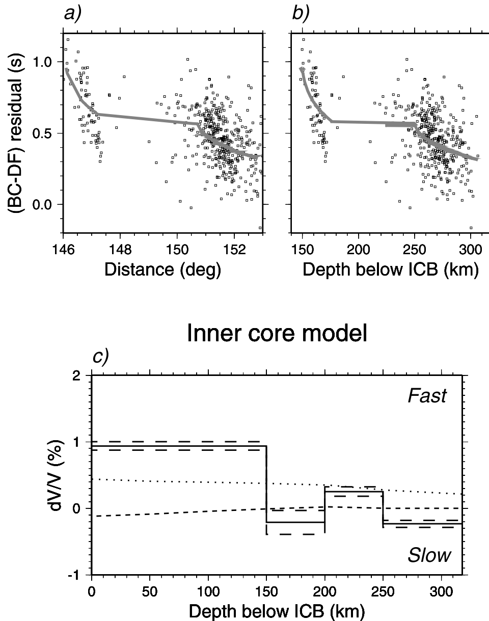
Figure 12. BC-DF differential travel time residuals for the ak135 Earth model and corresponding inner core model. (a) BC-DF differential travel time residuals are plotted as a function of epicentral distance and (b) maximum depth of the PKP(DF) rays in the inner core. Thick grey lines indicate BC-DF residuals predicted by the radial inner core model. (c) Velocity perturbation (%) as a function of depth in the inner core, obtained after inversion of the differential travel times residuals for an inner core model composed of four homogeneous layers. Solid and long dashed lines indicate the average and the standard deviation of the inner core velocity perturbation model, respectively. IASP91 (dotted line [Kennett and Engdahl, 1991]) and PREM (short dashed line [Dziewonski and Anderson, 1981]) inner core models are presented for comparison.
