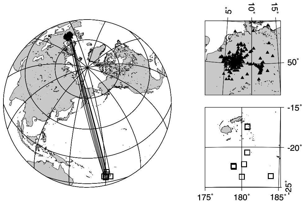
Figure 2. On the left, stations (solid triangles) and events (open squares) locations with typical great circle paths (solid lines). On the right, zoom of the (top) receiver and (bottom) source regions.
