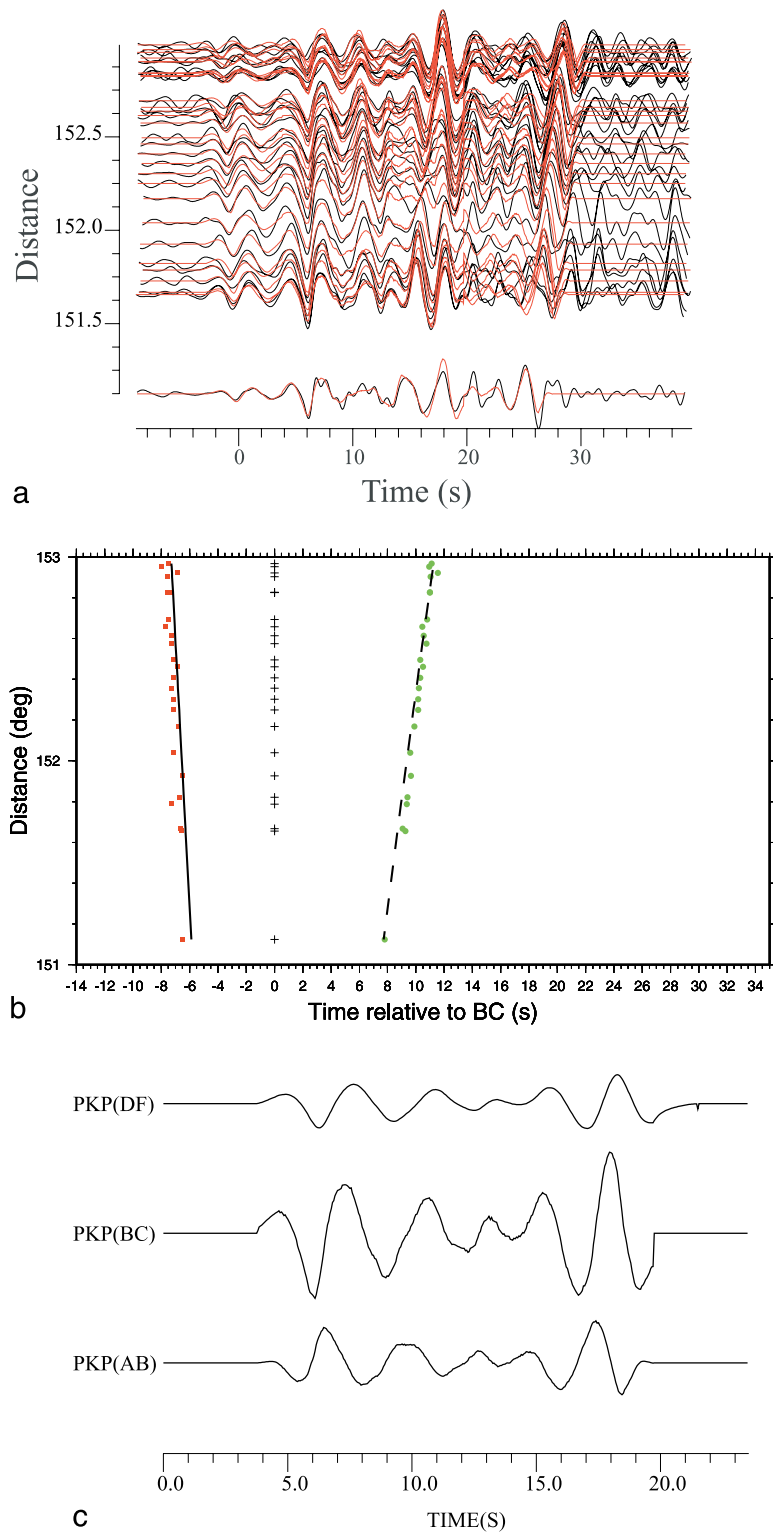
Figure 9. Example 3. (a) Data (black lines) and best model synthetic seismograms (red lines) aligned on the PKP(BC) phase. (b) Best model arrival times of the three PKP phases relative to PKP(BC) . Dashed lines indicate theoretical arrival times predicted by the ak135 reference Earth's model. (c) From top to bottom, waveforms obtained after inversions for PKP(DF) , PKP(BC) , and PKP(AB) phases as a function of time (s). Notice the two energy arrivals associated to direct and depth phases.
