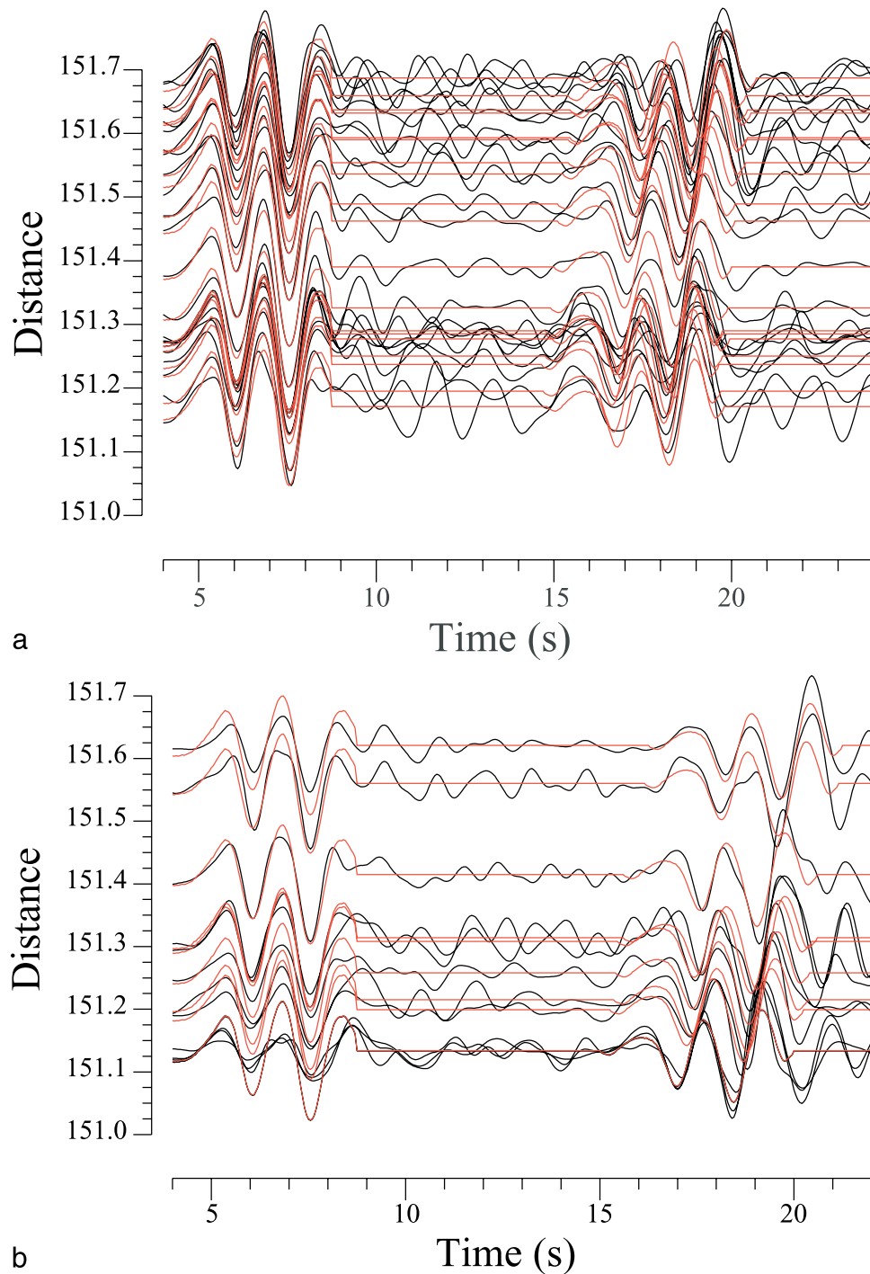
Figure 11. Closeup on the records of event 8 presenting (a) nominal PKP(AB) arrivals on top and (b) late arrivals on the bottom. Data (black lines) and synthetics (red lines) are aligned on the PKP(BC) phase seen on the left of the record sections. The PKP(AB) phase is properly fitted on both plots demonstrating that the larger AB-BC residuals are not due to cycle skipping problems. A similar pattern is observed for the AB-BC anomalous residuals of events 2 and 3.
