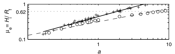
Figure 11. Effective friction \mu_e = H_i/R_f as a function of the aspect ratio a obtained from numerical simulation (circles) and from experiments (crosses). Best fit lines for the experimental data for an initial cone (solid lines) and the numerical experiments (dashed lines) have been added. The value of the friction coefficient \mu = \tan(32^\circ) = 0.62 is represented by a dotted line.
