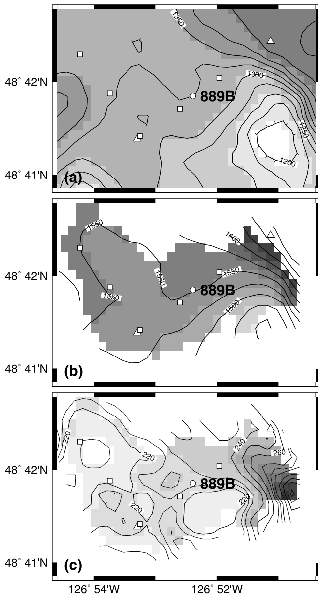
Figure 9. (a) Seafloor depth in the central part of the survey area. (b) BSR depth in the region where it is well-constrained (see text). (c) BSR depth below the seafloor in the region where it is well constrained. OBH positions and ODP Site 889 are marked as in Figure 1.
