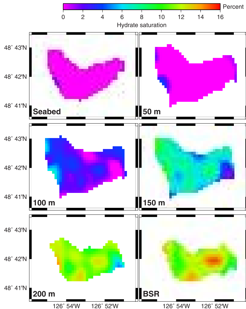
Figure 12. Hydrate content inferred for the depth slices of Figure 10, using the effective medium modeling approach of Jakobsen et al. [2000] (see text). The slice corresponding to velocities at the BSR is modeled using a porosity corresponding to 220 m depth below the seabed.
