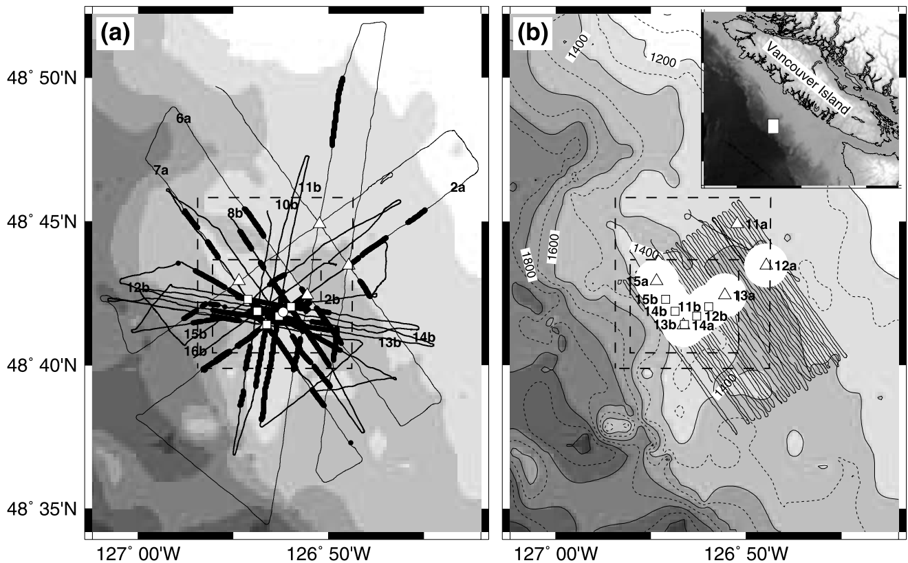
Figure 1. (a) Layout of OBH experiment. Grey scale marks bathymetry, with darker shades marking deeper water. Thin solid line marks shooting track during first OBH deployment, with triangles marking OBH positions. Thicker line marks shooting track during second OBH deployment, with squares marking OBH positions. Overlapping solid circles mark portions of the shooting track where BSR picks were made in coincident reflection profiles. Circle marks ODP Site 889. Profiles from which data are shown elsewhere in the paper are labeled. (b) Bathymetry marked as in Figure 1a but here also contoured at 100-m intervals. White circles around instrument positions mark approximately the regions where sediment velocities are constrained by refracted arrivals. Solid line marks shooting track for detailed reflection survey. Outer box marks region chosen for tomographic inversion; inner box marks well-constrained region chosen for the final run of the inversion.
