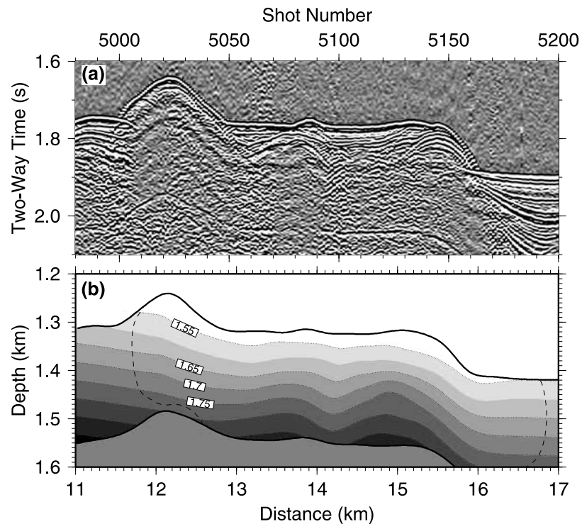
Figure 7. Comparison between (a) the deconvolved single channel reflection profile and (b) the final velocity model for line 2a. The dashed line marks the boundary of the well-constrained region of the velocity model (see text for discussion). The velocity structure close to the seabed follows the general trend of sedimentary reflectors, indicating that here velocities are controlled primarily by variations in porosity and lithology. Closer to the BSR this correlation is lost and velocities are likely controlled more by hydrate content.
