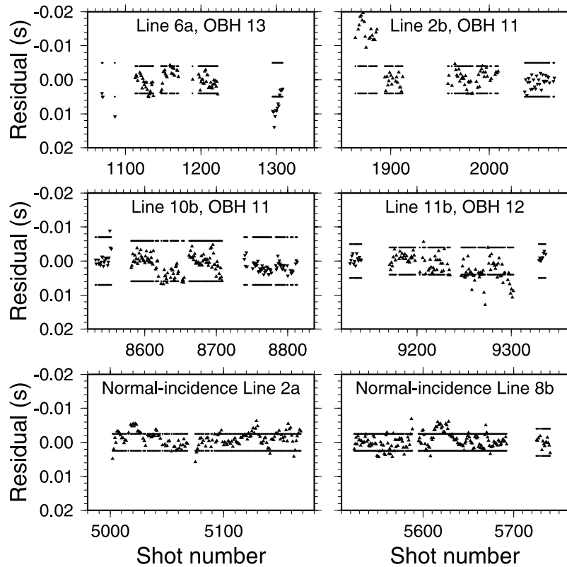
Figure 5. Typical residuals between observed and predicted travel times for the final model. Dots (which form broken horizontal lines) mark pick uncertainties, triangles mark residuals for BSR picks, and inverted triangles mark residuals for turning ray picks.
