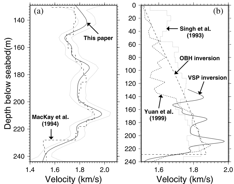
Figure 6. Velocity models at and close to ODP Site 889B. (a) Final result of VSP inversion (solid line), uncertainty bounds (dotted lines), and the result obtained by MacKay et al. [1994] (dashed line). (b) Result from VSP inversion (solid line), final result from OBH inversion (long-dashed line), result from waveform inversion of Yuan et al. [1999] (short-dashed line), and result from waveform inversion of Singh et al. [1993] (dotted line).
