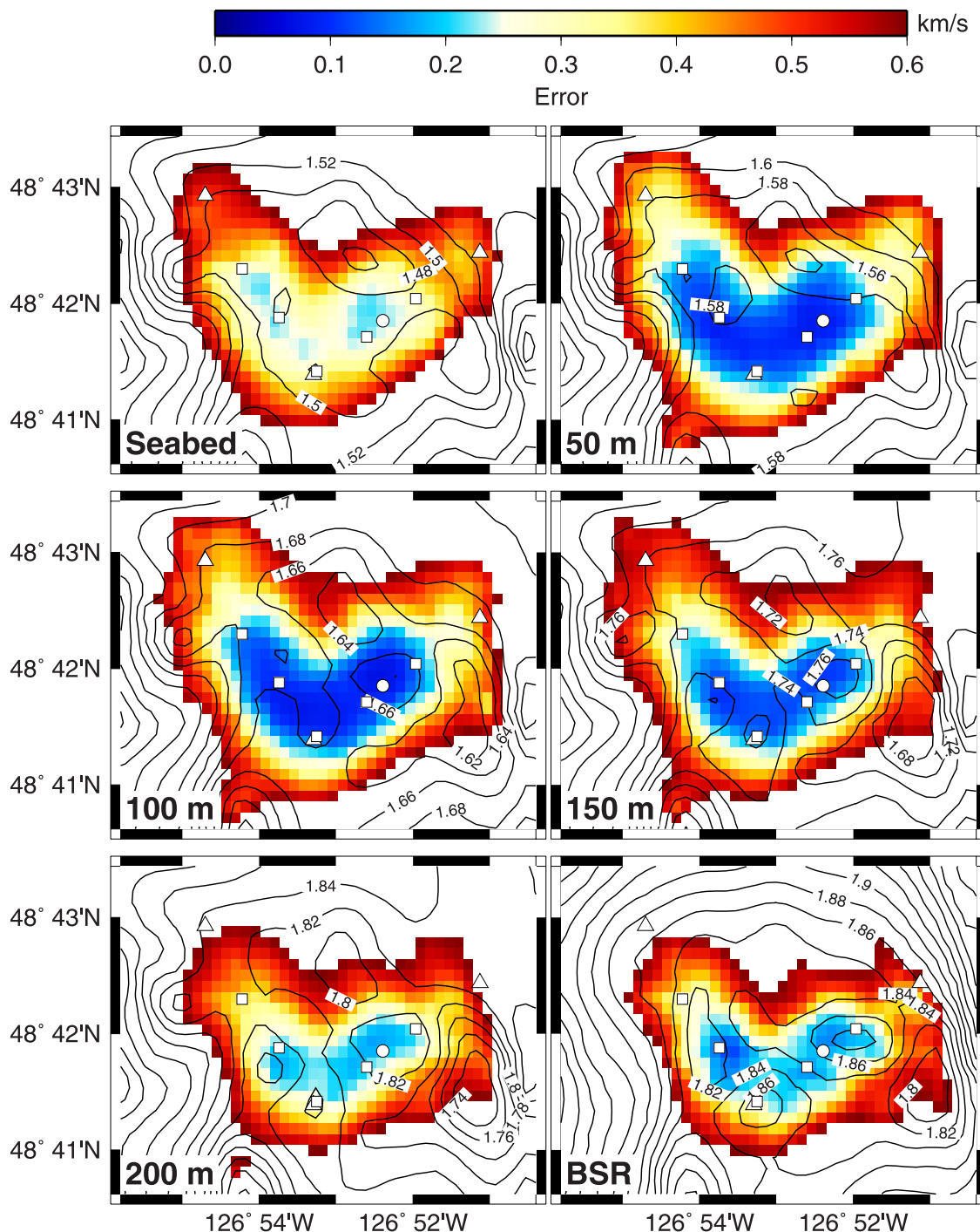
Figure 10. Representative slices through the final velocity model. Slices are shown at the seabed, at 50-m intervals through the hydrate stability zone and immediately above the BSR. Labeled contours mark velocities in \text{km s}^{-1} , and color scale marks the formal uncertainty from the inversion algorithm, which is likely overestimated by a factor of 2 or more (see text). The upper limit of the color scale marks the limit of the region which is considered to be well constrained (see text). OBH positions and ODP Site 889 are marked as in Figure 1.
