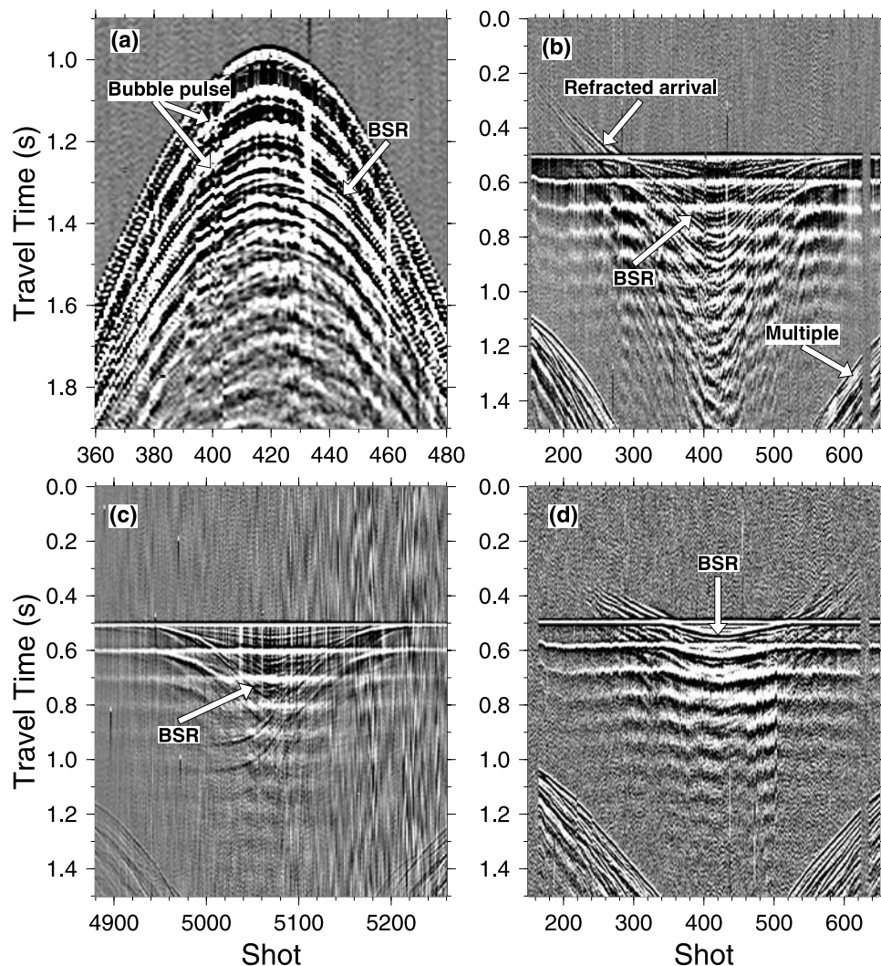
Figure 2. Representative OBH record sections. (a) Unreduced data from OBH12, deployment A. BSR is difficult to identify due to interfering bubble pulses from the direct arrival and to noise. (b) In-line data from OBH12, deployment A displayed with the direct arrival flattened. Strong BSR reflections are visible, and refracted energy both before and after the direct arrival. (c) In-line data from OBH14, deployment A, with a very weak BSR. (d) Off-line data from OBH13, deployment A showing a strong refracted energy before and after the direct arrival.
