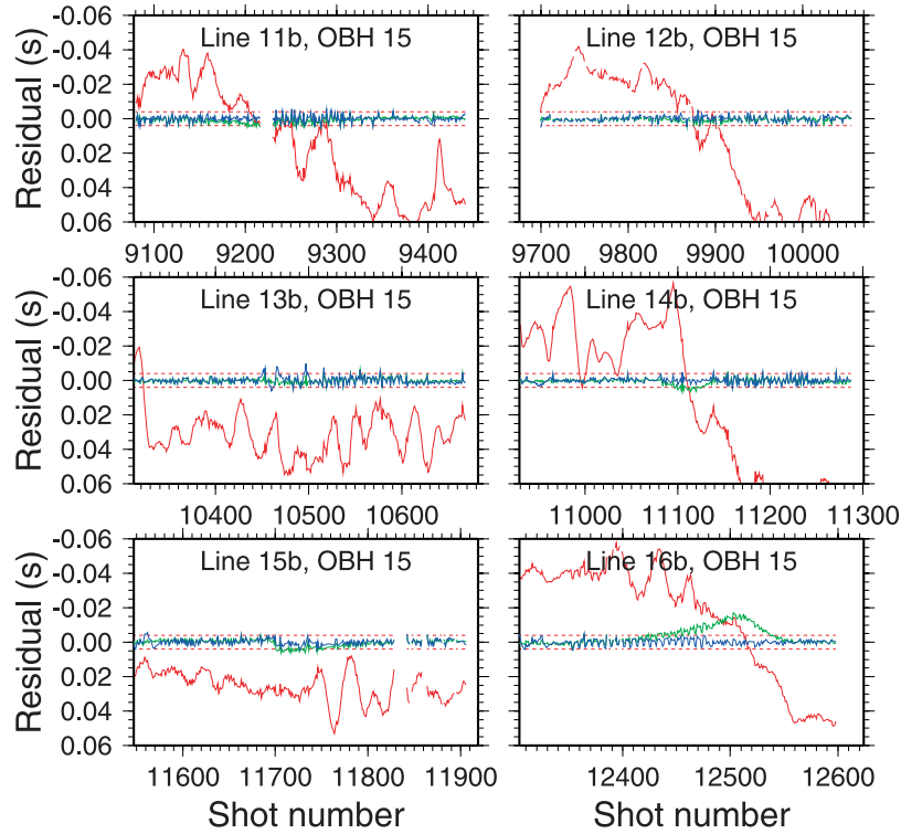
Figure 3. A selection of data and residuals for shot and instrument relocation, for the second OBH deployment. Travel time misfits are shown for the starting model (red), the model resulting from shot and instrument relocation (green), and the model resulting from a relocation algorithm in which static time shifts are also allowed (blue). Dashed lines show pick uncertainties.
