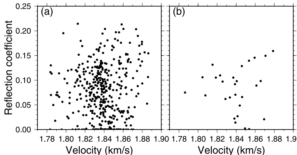
Figure 13. (a) BSR reflection coefficient as a function of the velocity immediately above the BSR, for the region where both are well constrained. Reflection coefficients are taken from Fink and Spence [1999], and the velocity grid was resampled at the interval of their reflection coefficient grid. (b) Same data resampled on a 500 m grid that is more representative of the horizontal resolution of the velocity model.
