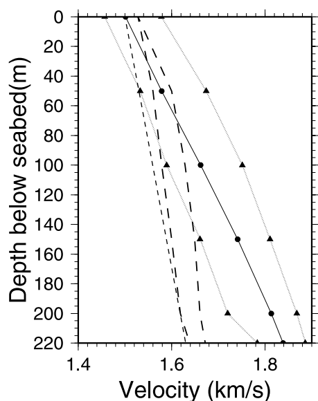
Figure 11. Mean velocity in the constrained region for each of the slices shown in Figure 10 (circles) and maximum and minimum velocity in the constrained region of each slice (triangles). Velocities at the BSR are plotted at a depth of 220 m below the seafloor. Short-dashed line marks no-hydrate reference curve of Yuan et al. [1996]. Long-dashed lines mark the velocity computed using the approach of Jakobsen et al. [2000] for the best fitting exponential porosity-depth relation (higher values) and the upper limit of porosity from the borehole porosity log at Site 889 (lower values).
