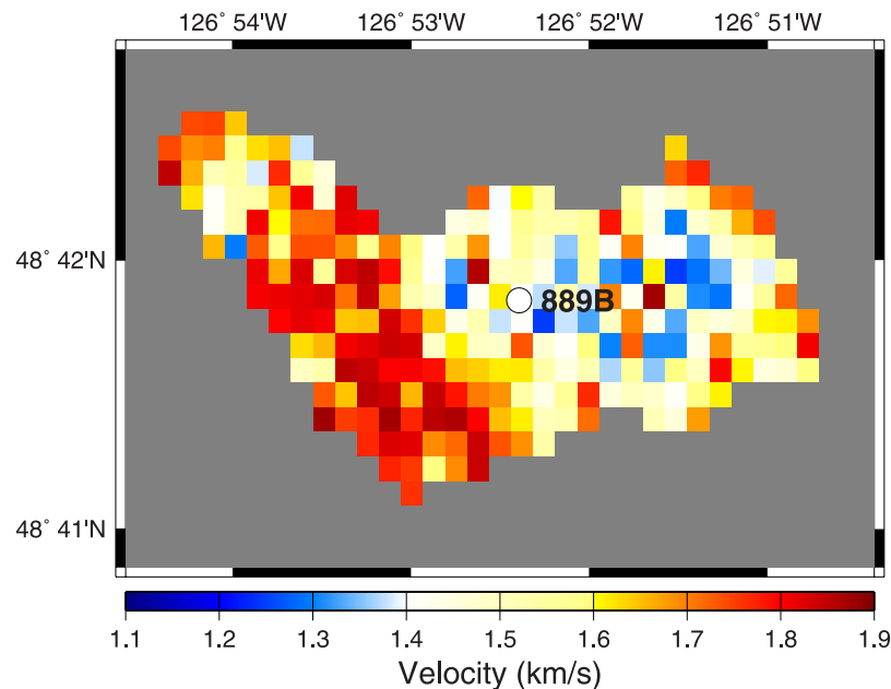
Figure 14. Seismic velocity immediately beneath the BSR, inferred from the reflection coefficient grid of Fink and Spence [1999] and the velocity immediately above the BSR from tomographic inversion, assuming that there is no density contrast at the BSR.
