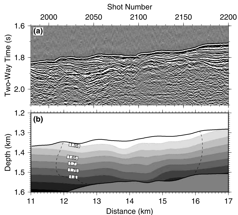
Figure 8. Comparison between (a) the deconvolved single channel reflection profile and (b) the final velocity model for line 7a, with the boundary of the well-constrained region as in Figure 7.
