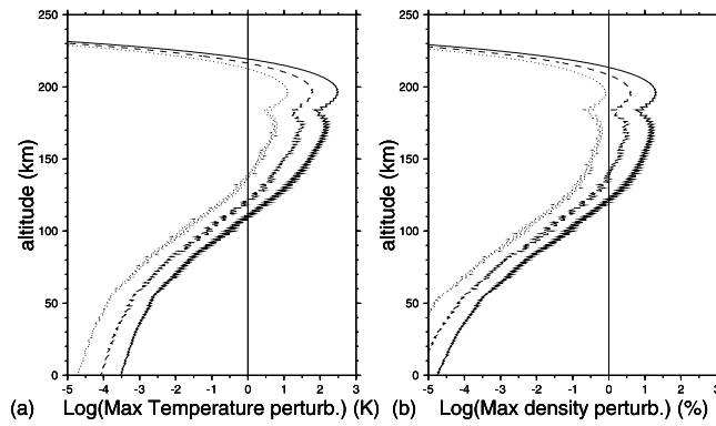
Figure 3. Logarithm of (a) the maximum adiabatic temperature perturbation (in K) and (b) the maximum density perturbation (in %), just above the source, as a function of altitude (in km) for different earthquake magnitudes: M5.0 (dotted line), M5.5 (dashed line) and M6.0 (plain line). Vertical bars are visual guides at 1K and 1% levels.
