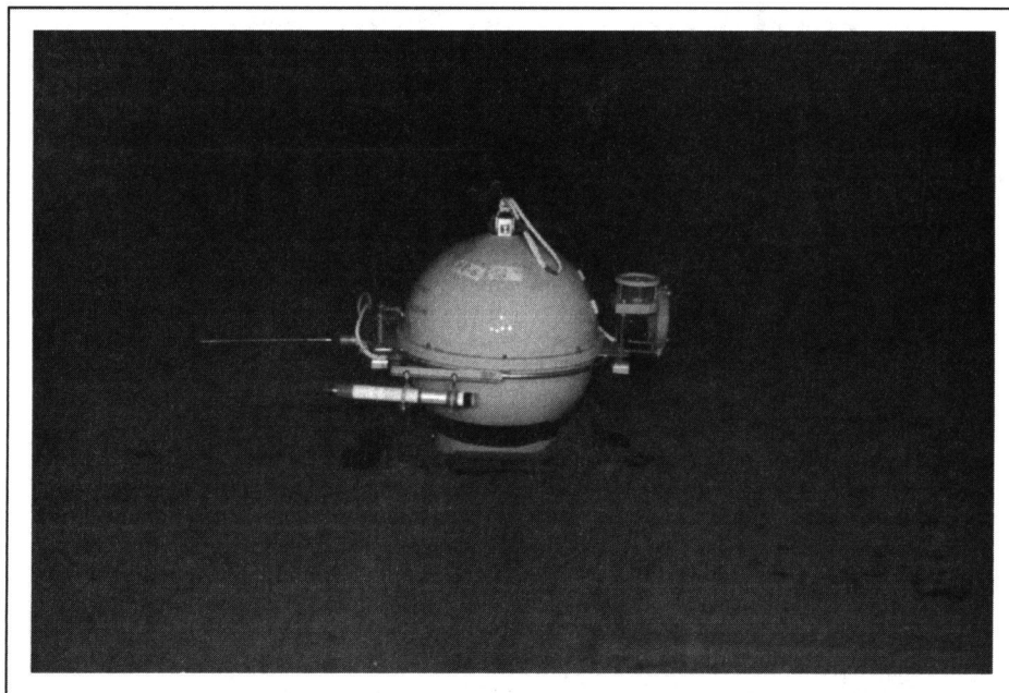
Fig. 2. The BBOBS on the seafloor at the FP6 station, which is 200 km south of the Macdonald hot spot at a depth of 4400 m. Original color image appears at the back of this volume.
