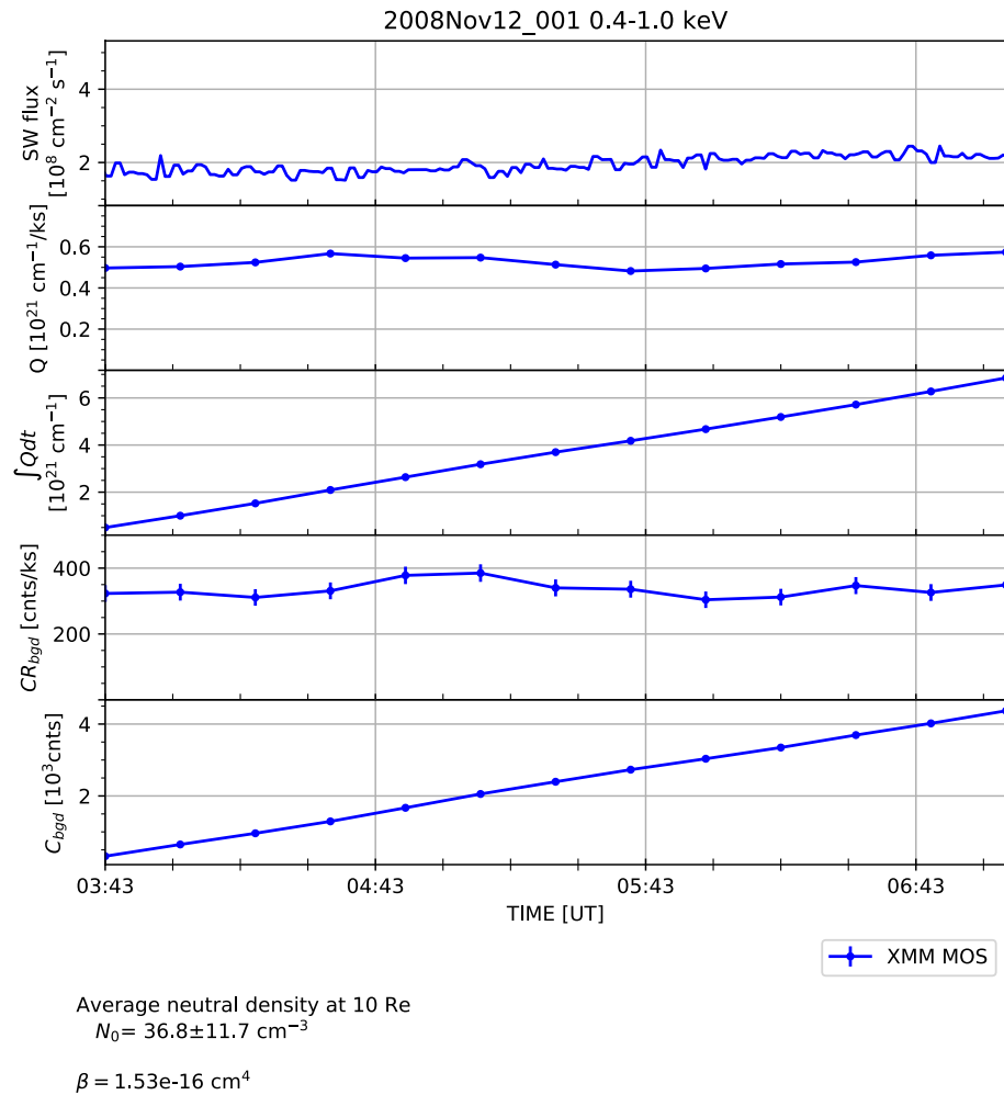
Figure 5. Modeled potential reaction rate and total XMM background counts of the 12 November 2008 event. From top to bottom, the solar wind flux, modeled potential reaction rate ( Q ), accumulated potential reaction rate ( \int Q dt ), total XMM background count rate ( CR_{bgd} ), and accumulated XMM count rates ( \int C_{bgd} ) are shown. The effective scale factor \beta is shown at the bottom of the figure.
