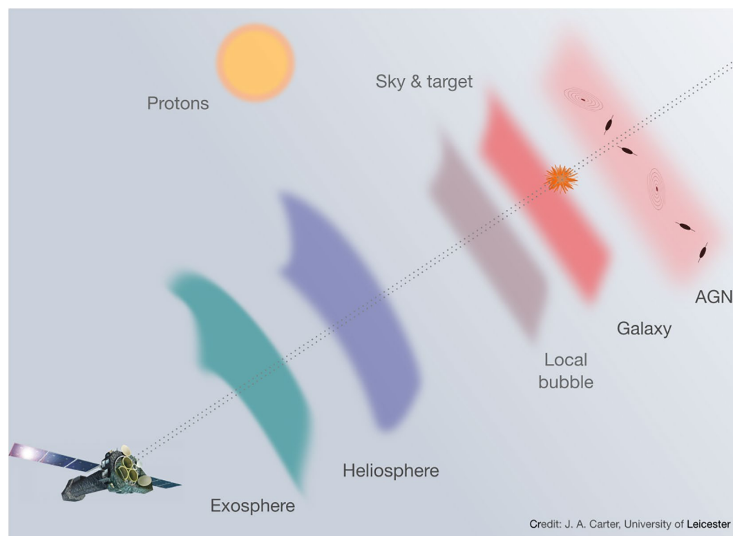
Figure 1. Various X-ray signals and the soft protons that create false counts in X-ray Multimirror Mission X-ray cameras.
