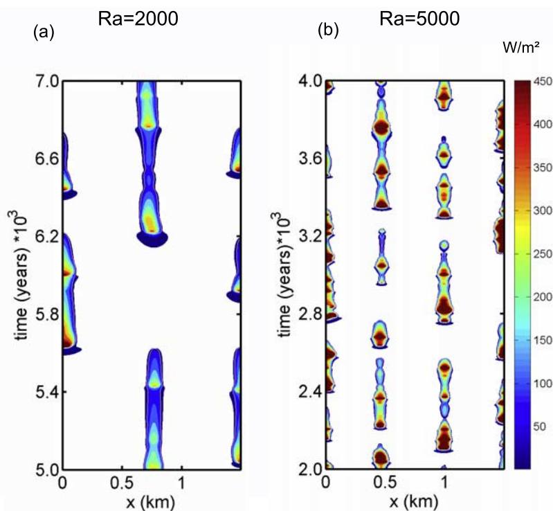
Figure 5. (a) Temporal variations of the heat flux ( \text{W/m}^2 ) at different locations on the seafloor for the model of Figure 4, which has a permeability of k = 4 \cdot 10^{-15} \text{ m}^2 ( Ra = 2000 ). The shaded areas correspond to the heat flux of each individual venting sites; the white areas correspond to zones of downflow. Overprinted white lines represent the 300^\circ\text{C} isotherm. A large part of the fluid vents at temperatures >300^\circ\text{C} . Corresponding heat flux ranges from \sim 50 \text{ W/m}^2 to 200 \text{ W/m}^2 . Note that when the plume located on the left side stops short of the surface, the heat flux of the “middle” plume increases. (b) Same as Figure 5a but for the model of Figure 6, which has a permeability of 10^{-14} \text{ m}^2 ( Ra = 5000 ). The heat flux ranges from 100 \text{ W/m}^2 to >400 \text{ W/m}^2 .
