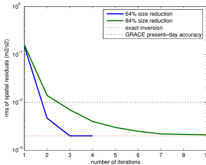
Fig. 8. Evolution of the rms of the spatial residuals between the simulated data and the reconstructed data as a function of the iteration number in the cases: 64% size reduction, 84% size reduction, no size reduction.
