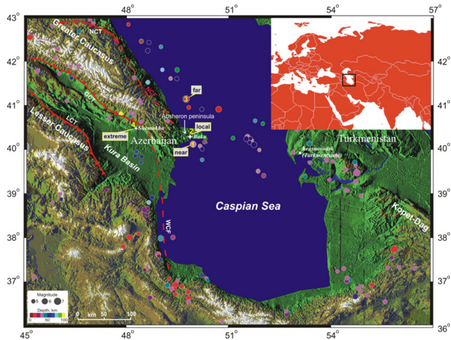
Fig. 1. Topography, simplified tectonics, and seismicity of the Caucasus to the Kopet-Dag region. The inset presents a map of central Eurasia showing the region's location. Earthquake epicenters are marked by circles, and the colours of the circles provide information on the depth of the earthquake hypocenters (earthquakes of magnitude 5 and greater for the period of 1950–2006 are plotted here). Target earthquakes are marked by numbers: (1), the 2000 M = 6.3 Caspian earthquake; (2), the 1935 M = 3.5 Surakhani earthquake; (3), the 1963 M = 6.5 Caspian earthquake; and (4), the hypothetical extreme event in Shemakha. Abbreviations: NCT, North Caucasus thrust fault; GCT, Greater Caucasus thrust fault; LCT, Lesser Caucasus thrust fault; WCF, West Caspian fault; and NCF, North Caspian fault.
