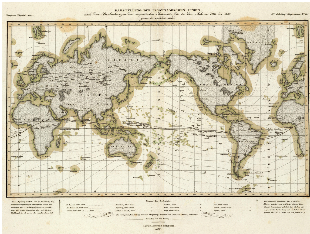
Figure 7. World map of isodynamics of intensity measured in 1790–1830 published in Gotha in 1837. The values are given in relative “Humboldt units”, magnetic equator is marked with a bold line (Berghaus, 1837–1848) (David Rumsey Map Collection, www.davidrumsey.com, USA; Images copyright © 2000 by Cartography Associates).
