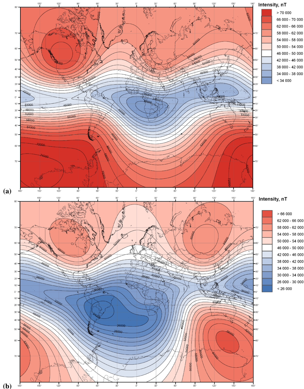
Figure 3. Observed magnetic field fading comparing maps of total intensity isodynames for 1600 (a) and 2000 (b).
