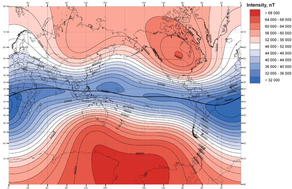
Figure 10. World map of total intensity for 1830 calculated according to gufm1 model. Magnetic equator is marked with a bold line.
