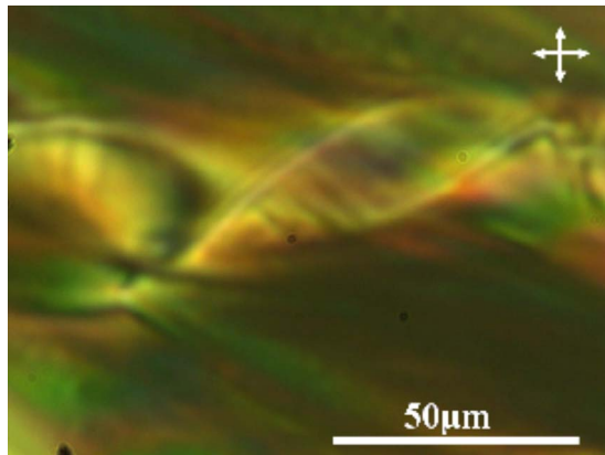
FIG. 9. (Color online) Helical ribbon in cholesteryl nonanoate (C9) with its axis parallel to the polarizer. The dark background indicates that outside the helical ribbon the smectic layers are perpendicular to the axis of the helical ribbon.
