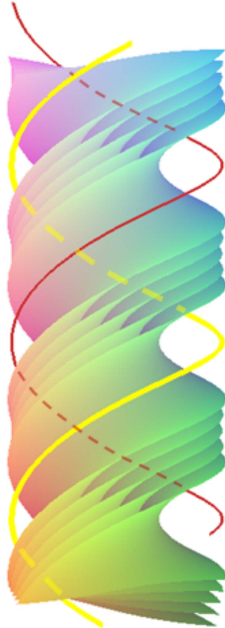
FIG. 1. (Color online) Parallel helicoidal surfaces inside C and their two cuspidal lines modeling an arrangement of smectic layers with two helical disclinations, for a giant Burgers vector dislocation in its split mode; p=2nd_0 . For clarity one of the disclinations (yellow/light gray) is shown thicker than the other one (red/gray dark).
