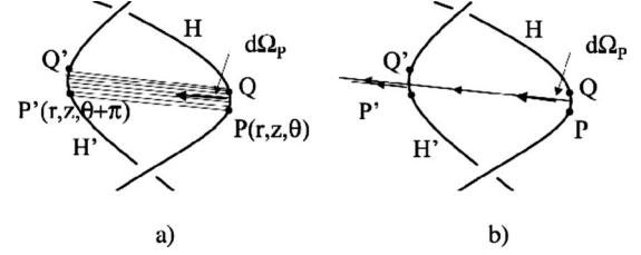
FIG. 7. (a) Disclination densities of rotation vectors d\Omega_P in the N^* phase, attached between P and Q=P+dP on H , P' , and Q'=P'+dP on H' ; they form a stacking fault between H and H' . The helices H and H' are at the same constant distance \rho=r_H=r_{H'} of the central axis. The rotation vectors \Omega_P, \Omega_{P'}, \Omega_Q, \dots tangent to H and H' are not represented. (b) Cancellation outside the stacking fault of infinitesimal disclination lines attached to PQ and P'Q' at opposite points on H and H' ; these disclinations have the same orientation, but opposite rotation vectors.
