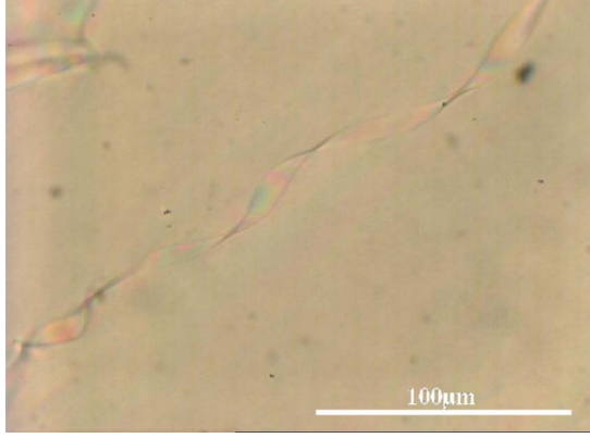
FIG. 6. (Color online) DH^* in a C9 sample; the Darboux condition is not obeyed.
