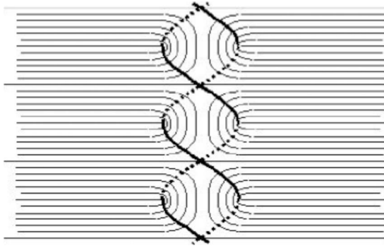
FIG. 2. Sketch of the smectic layers (thin lines) inside and outside C and double helical disclinations (thick lines) in a DH. In reality, the double helix is much distorted in a Sm-A, but the topology is the same. Isometry is globally preserved, as explained in Sec. V.
