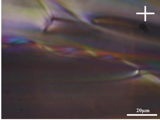
FIG. 8. (Color online) Helical ribbon associated with a parabolic FCD. Type II specimen, C9.
