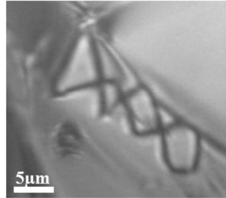
FIG. 4. Darboux's condition obeyed for a DH in Sm-A of 8CB.
