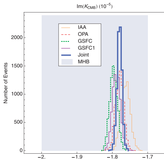
Figure 2. Marginal posterior pdf of \text{Im}(K_{\text{CMB}}) for the individual inversion of the three time-series (GSFC, OPA and IAA), the joint inversion (Joint) and for the GSFC data truncated to the period 1990–2009.3 (GSFC1). The blue box is the 99.7 per cent CI obtained by Mathews et al. (2002) (MHB).
