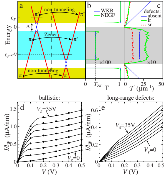
FIG. 2. (Color online) Electronic transport in graphene: theory. (a) Electronic bands of L and R contacts. The hyperbolae are the bands corresponding to a finite k_{\perp} ( \Delta = 2\hbar v_F k_{\perp} = 22 meV). In L and R contacts the bands are filled up to \epsilon_F and \epsilon_F - eV , respectively, where \epsilon_F > 0 ( \epsilon_F < 0 ) corresponds to electron (hole) doping. [(b) and (c)] Electronic transmissions T and \bar{T} , defined as in Eq. (1), for V = 0.1 V and l = 1 \mu\text{m} . In the gray zone (the region corresponding to the Zener-Klein tunneling) T and \bar{T} are magnified. (b) Ballistic case calculated with NEGF or with the WKB approximation. (c) NEGF results in the ballistic case (no defects) or in the presence of lr or sr defects. [(d) and (e)] calculated current I per unit of lateral length l_W vs V (the voltage applied between the electrodes) as a function of the gate voltage ( V_g ). V_g goes from 0 to 35 V with 5 V step, l = 1 \mu\text{m} . In the ballistic case (d), lines are approximated semiclassical results (i.e., the analytical curves from Appendix A), points are from the exact NEGF simulations.
